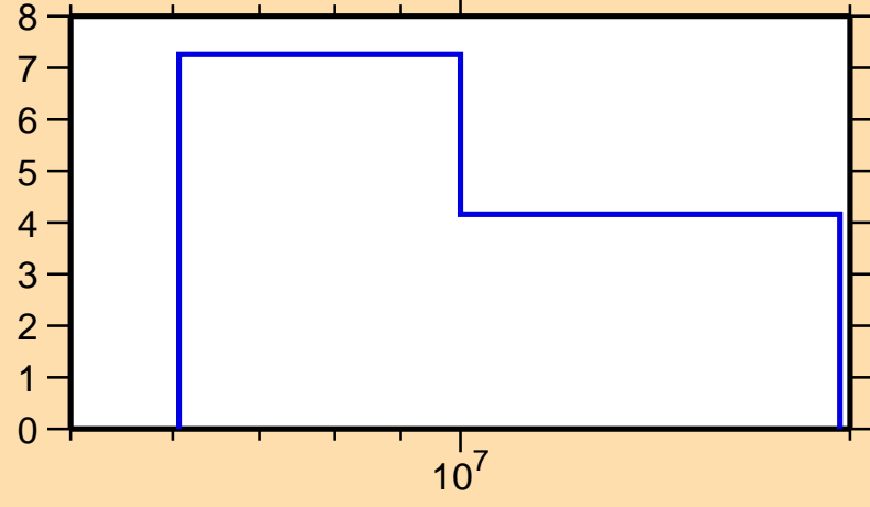
\Delta\sigma/\sigma vs. E for ^{201}\text{Hg}(n,\text{tot.})
