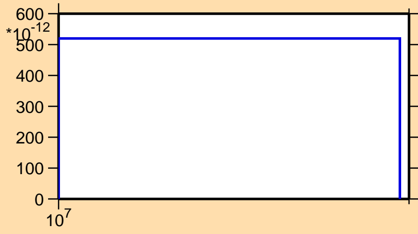
\sigma vs. E for ^{201}\text{Hg}(n,\text{nd})
