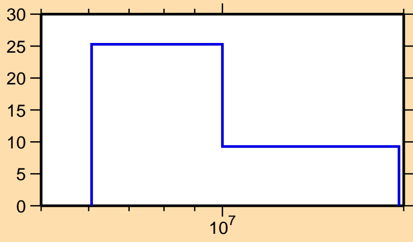
\Delta\sigma/\sigma vs. E for ^{201}\text{Hg}(n,2n)
