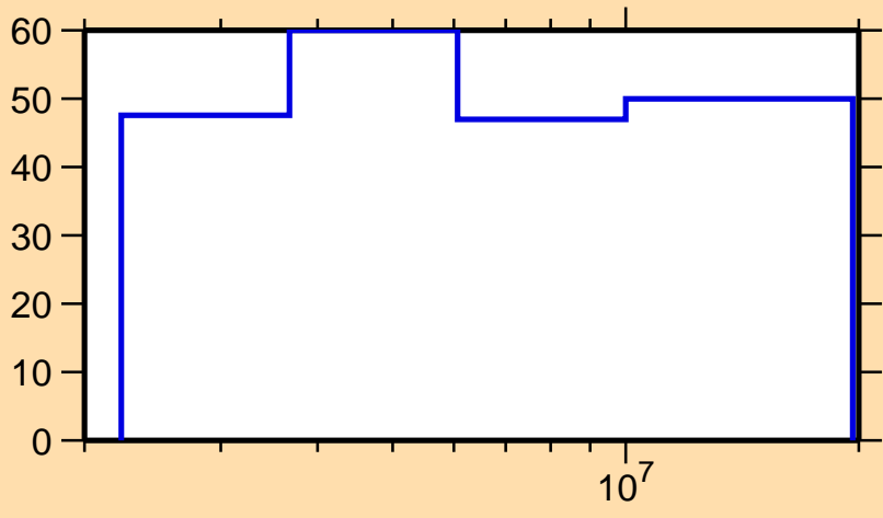
\Delta\sigma/\sigma vs. E for ^{201}\text{Hg}(n,p)
