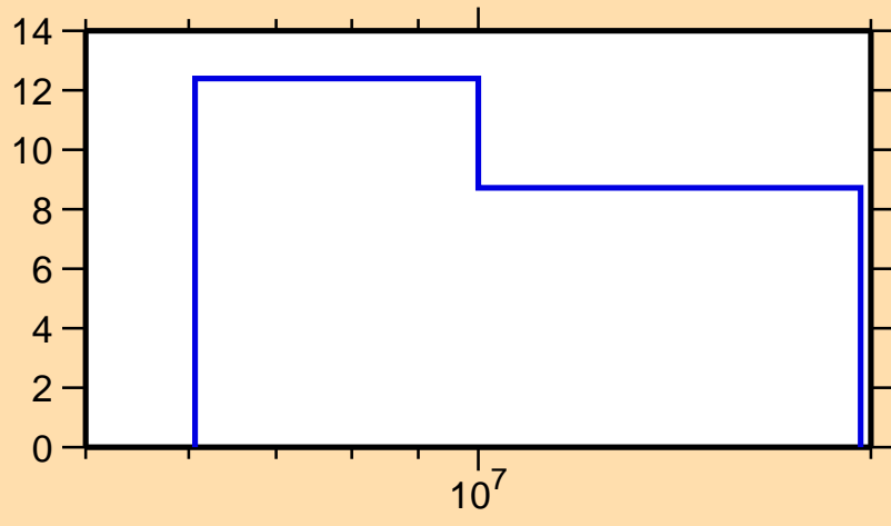
\Delta\sigma/\sigma vs. E for ^{201}\text{Hg}(n,\text{el.})
