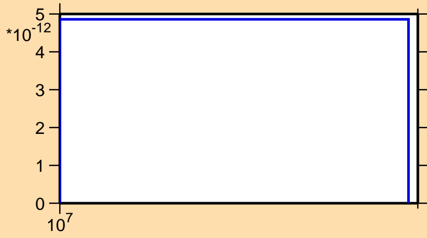
\sigma vs. E for ^{201}\text{Hg}(n,nt)
