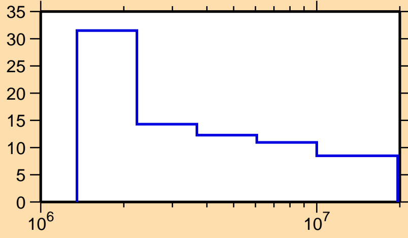
\Delta\sigma/\sigma vs. E for ^{201}\text{Hg}(n,n\text{onel.})
