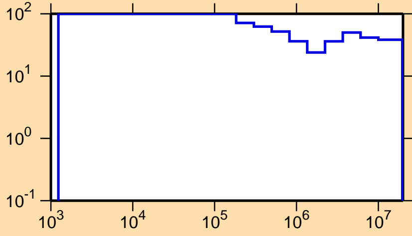
\Delta\sigma/\sigma vs. E for ^{201}\text{Hg}(n,n_1)
