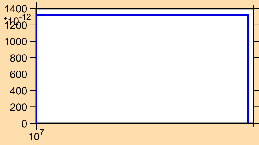
\sigma vs. E for ^{201}\text{Hg}(n,2n\alpha)
