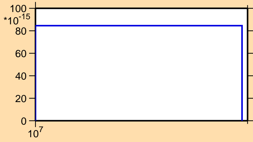
\sigma vs. E for ^{201}\text{Hg}(n,\text{He}3)
