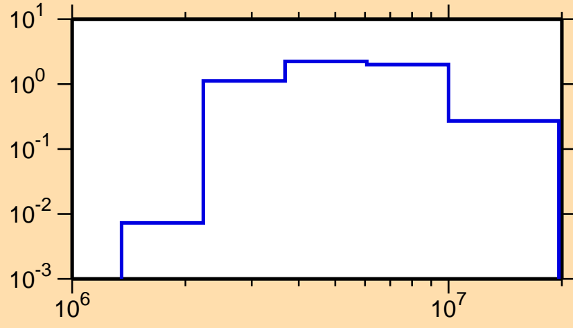
\sigma vs. E for ^{201}\text{Hg}(n,n\text{cont.})
