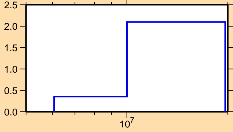
\sigma vs. E for ^{201}\text{Hg}(n,2n)
