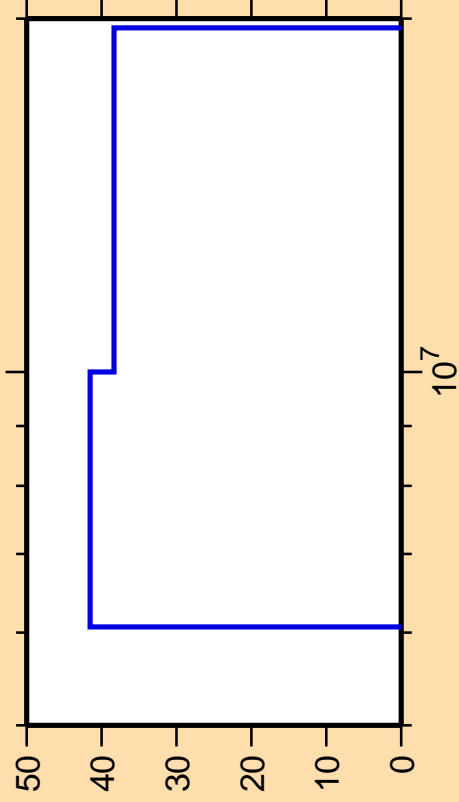
\Delta\sigma/\sigma vs. E for ^{201}\text{Hg}(n,n_1)
