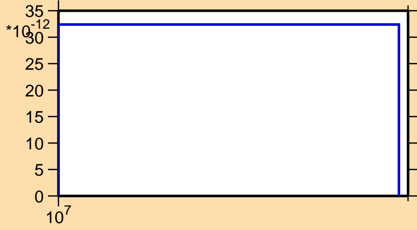
\sigma vs. E for ^{201}\text{Hg}(n,2np)
