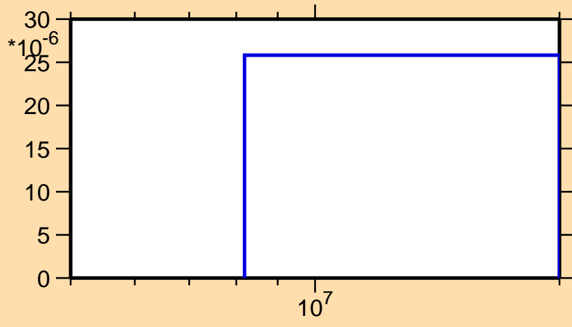
\sigma vs. E for ^{201}\text{Hg}(n,np)
