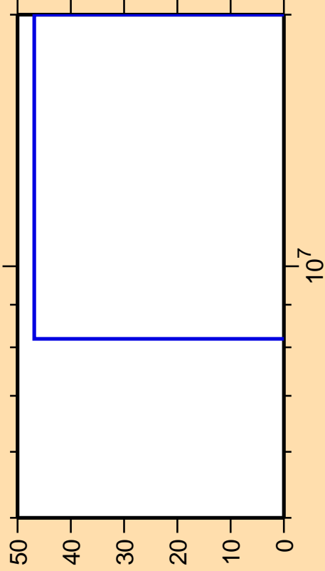
\Delta\sigma/\sigma vs. E for ^{201}\text{Hg}(n,np)
