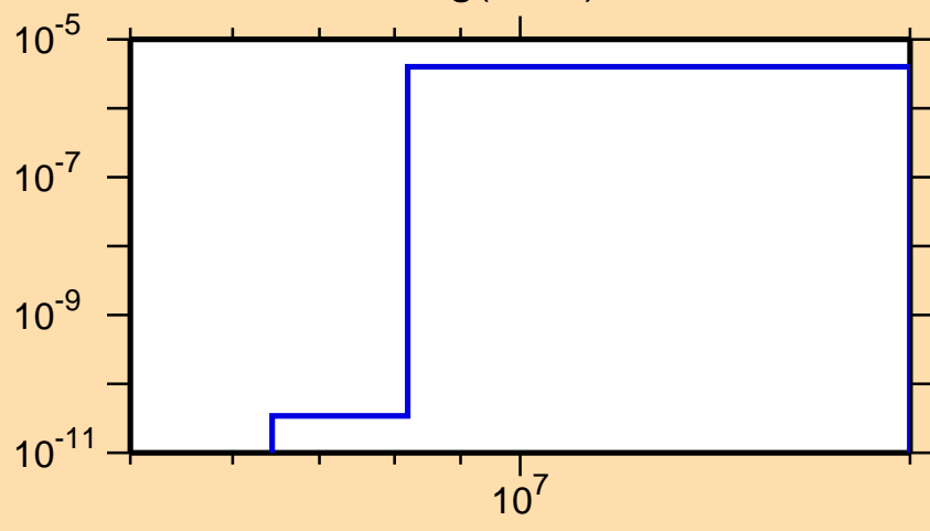
\sigma vs. E for ^{201}\text{Hg}(n,n\alpha)
