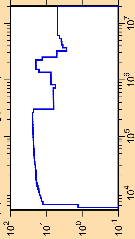
\Delta\mu/\mu vs. E for ^{202}\text{Hg}(\text{mt251})
