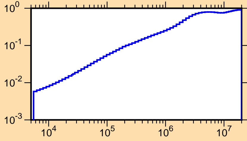
\mu vs. E for ^{202}\text{Hg}(\text{mt251})
