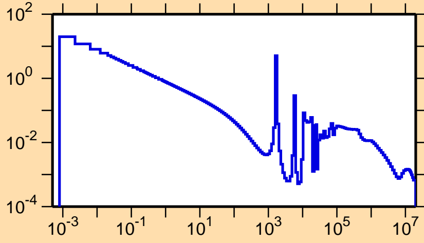
\sigma vs. E for ^{202}\text{Hg}(n,\gamma)
