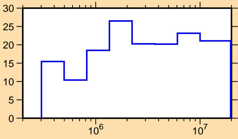
\Delta\sigma/\sigma vs. E for ^{202}\text{Hg}(n,n_1)
