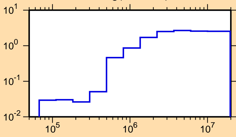
\sigma vs. E for ^{202}\text{Hg}(n,\text{nonel.})
