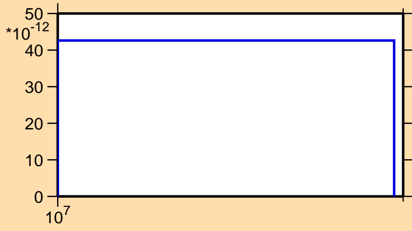
\sigma vs. E for ^{202}\text{Hg}(n,2n\alpha)
