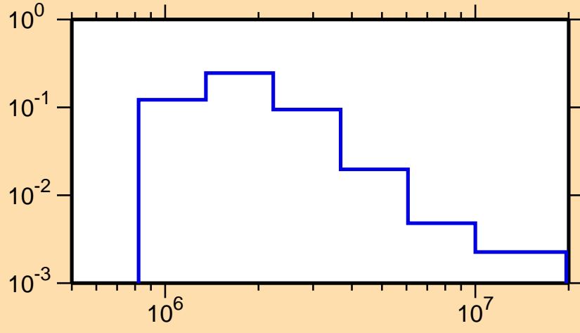
\sigma vs. E for ^{202}\text{Hg}(n,n_2)
