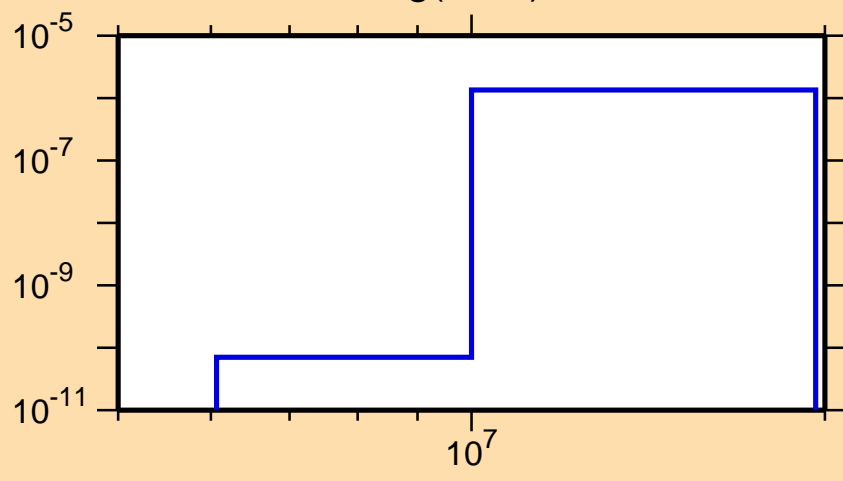
\sigma vs. E for ^{202}\text{Hg}(n,n\alpha)
