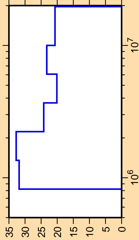
\Delta\sigma/\sigma vs. E for ^{202}\text{Hg}(n,n_3)
