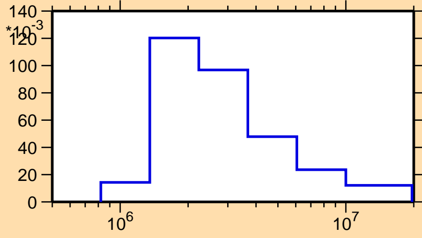
\sigma vs. E for ^{202}\text{Hg}(n,n_3)
