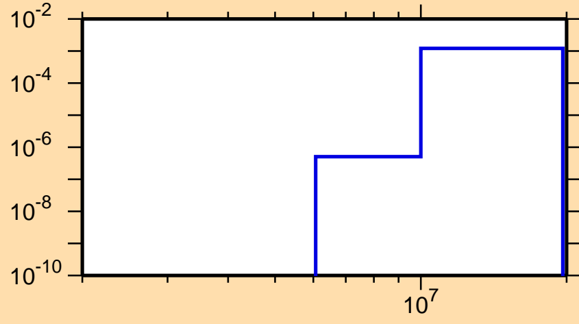
\sigma vs. E for ^{202}\text{Hg}(n,p)
