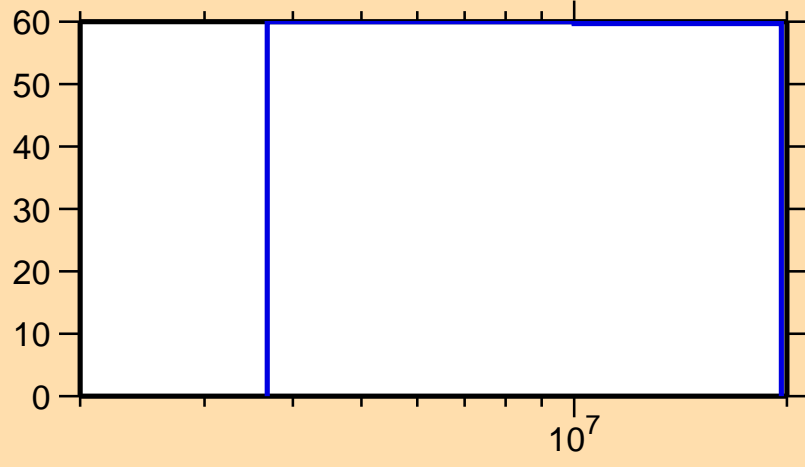
\Delta\sigma/\sigma vs. E for ^{202}\text{Hg}(n,p)
