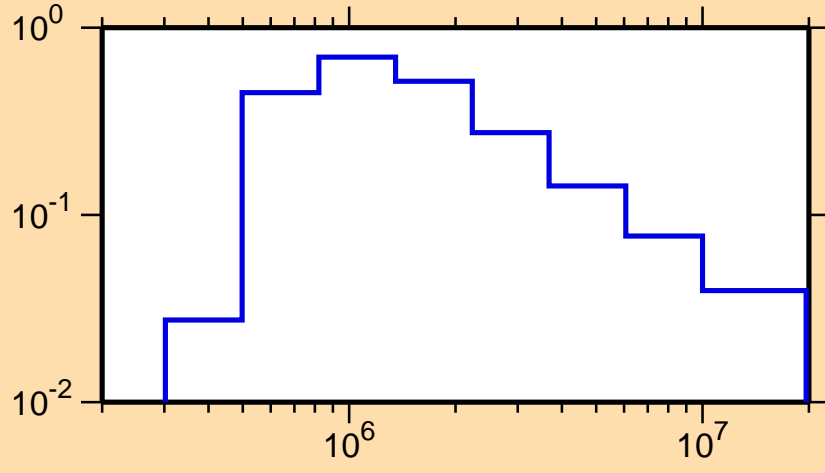
\sigma vs. E for ^{202}\text{Hg}(n,n_1)
