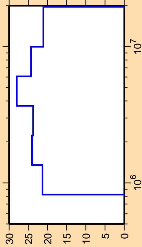
\Delta\sigma/\sigma vs. E for ^{202}\text{Hg}(n,n_2)
