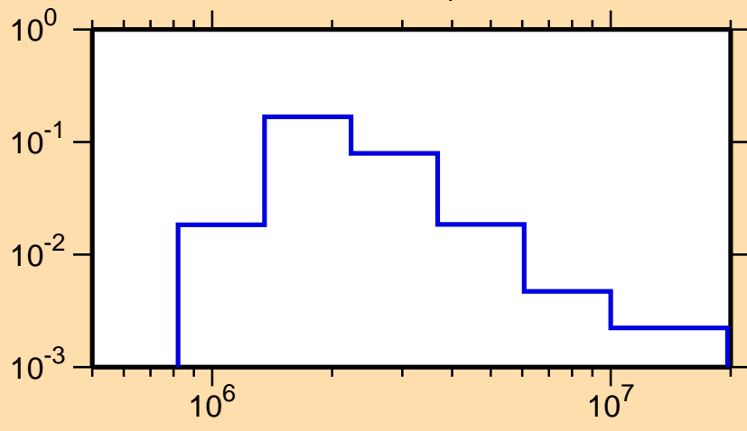
\sigma vs. E for ^{202}\text{Hg}(n,n_4)
