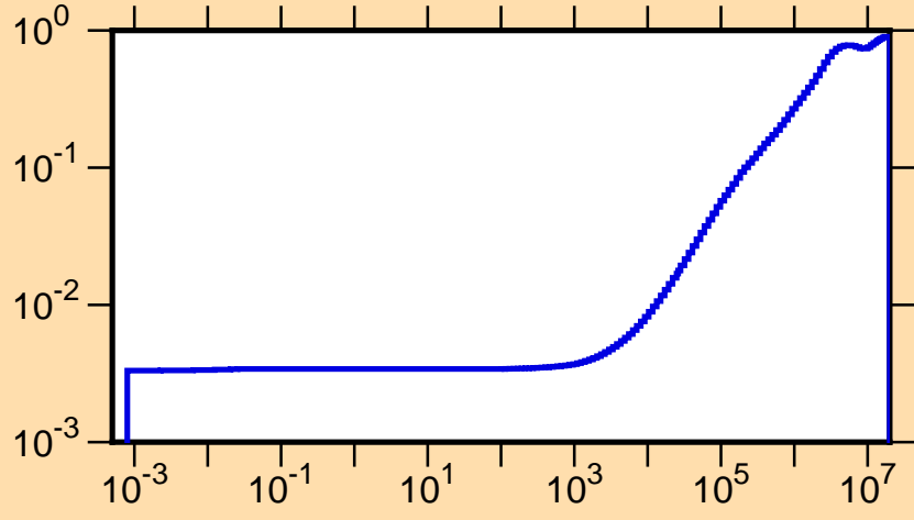
\mu vs. E for ^{203}\text{Hg}(\text{mt251})
