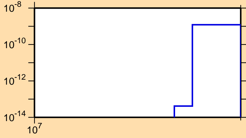
\sigma vs. E for ^{203}\text{Hg}(n,nt)
