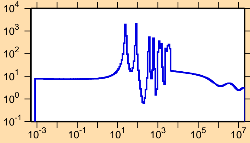
\sigma vs. E for ^{203}\text{Hg}(n,\text{el.})
