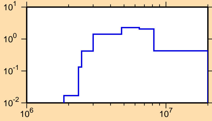
\sigma vs. E for ^{203}\text{Hg}(n,n\text{cont.})
