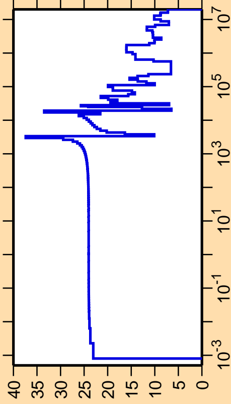
\Delta\sigma/\sigma vs. E for ^{204}\text{Hg}(n,\text{el.})
