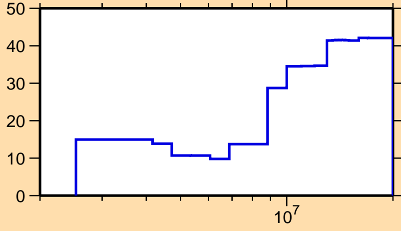
\Delta\sigma/\sigma vs. E for ^{204}\text{Hg}(n,n\text{cont.})
