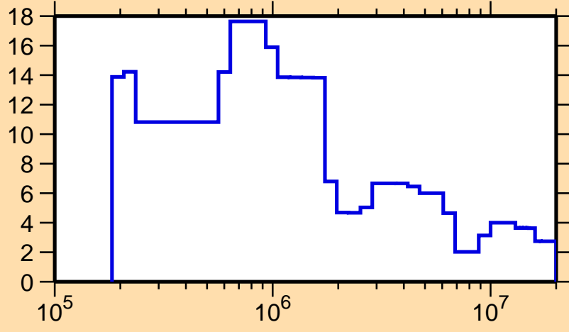
\Delta\sigma/\sigma vs. E for ^{204}\text{Hg}(n,\text{tot.})
