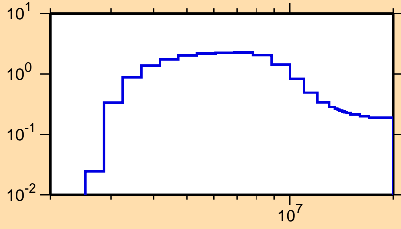
\sigma vs. E for ^{204}\text{Hg}(n,n\text{cont.})
