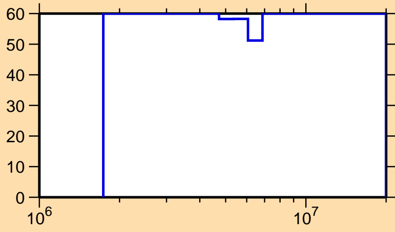
\Delta\sigma/\sigma vs. E for ^{205}\text{Hg}(n,\gamma)
