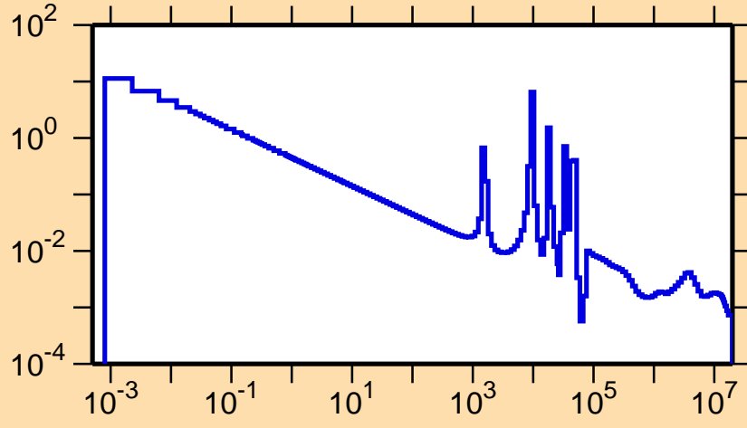
\sigma vs. E for ^{205}\text{Hg}(n,\gamma)
