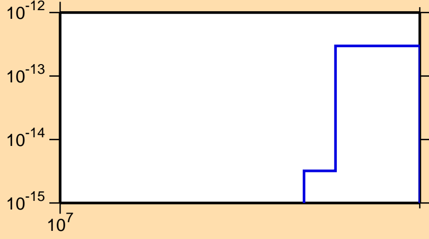
\sigma vs. E for ^{205}\text{Hg}(n,p\alpha)
