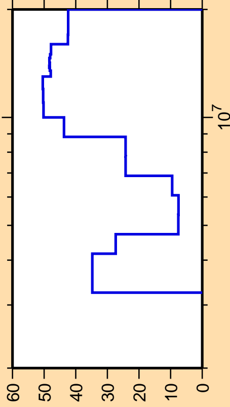
\Delta\sigma/\sigma vs. E for ^{205}\text{Hg}(n,n\text{cont.})
