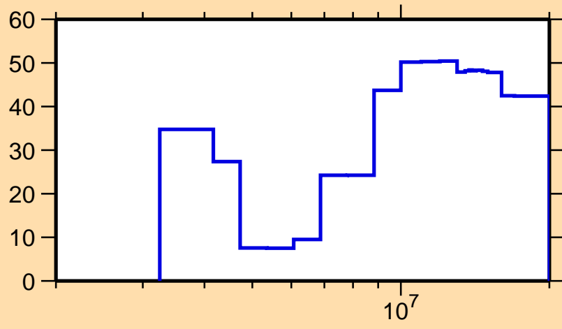
\Delta\sigma/\sigma vs. E for ^{205}\text{Hg}(n,n\text{cont.})
