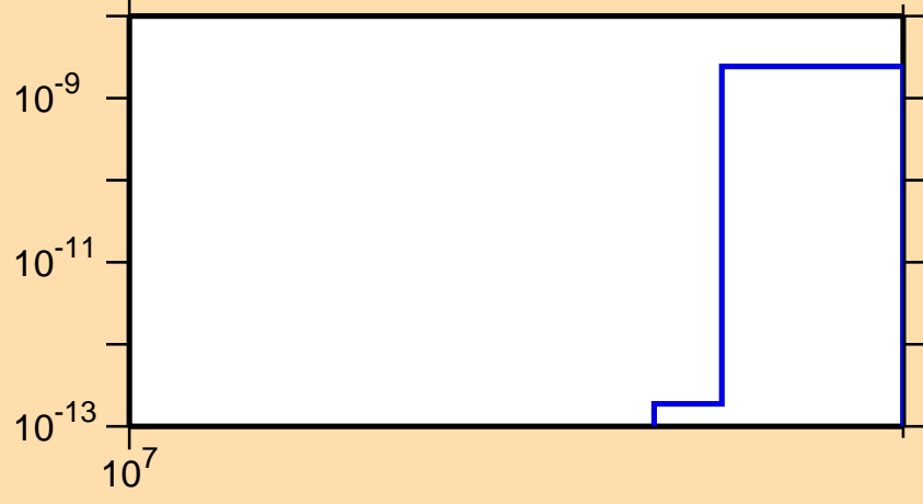
\sigma vs. E for ^{205}\text{Hg}(n,nt)
