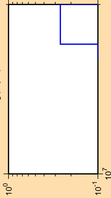
\Delta\sigma/\sigma vs. E for ^{205}\text{Hg}(n,p\alpha)
