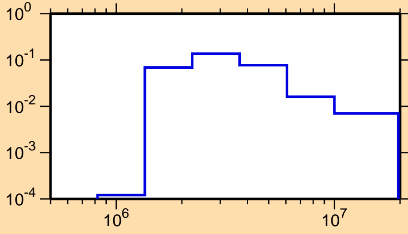
\sigma vs. E for ^{205}\text{Hg}(n,n_4)
