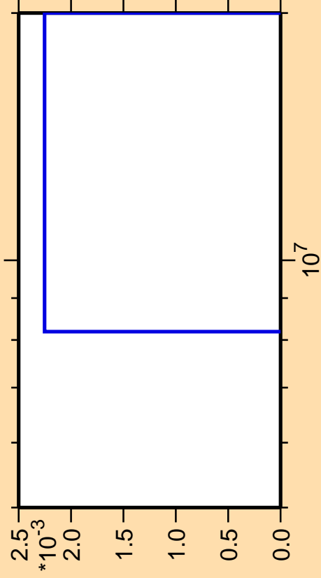
\Delta\sigma/\sigma vs. E for ^{205}\text{Hg}(n,p\alpha)
