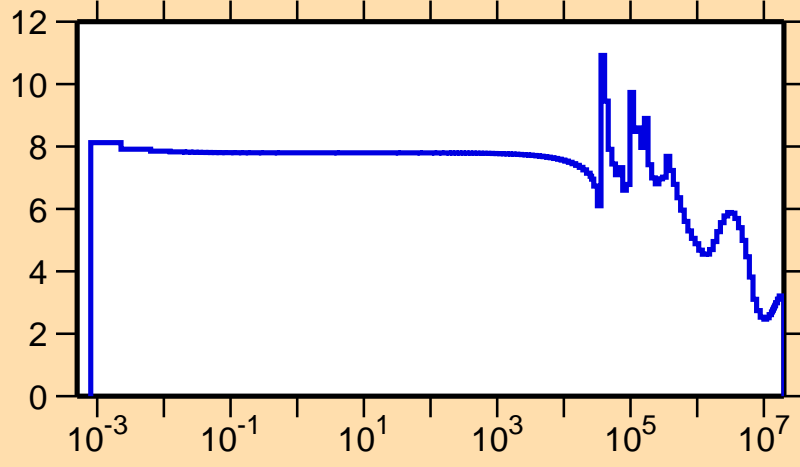
\sigma vs. E for ^{206}\text{Hg}(n,\text{el.})
