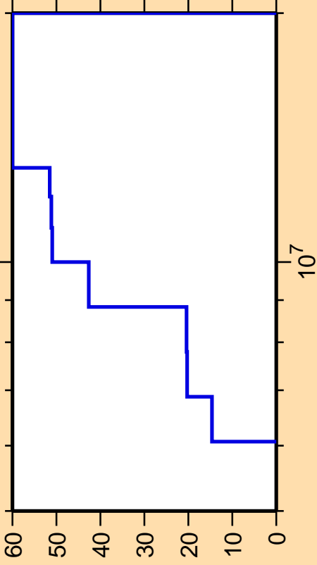
\Delta\sigma/\sigma vs. E for ^{206}\text{Hg}(n,n\text{cont.})
