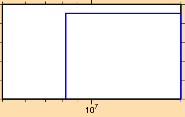
\sigma vs. E for ^{206}\text{Hg}(n,2np)
