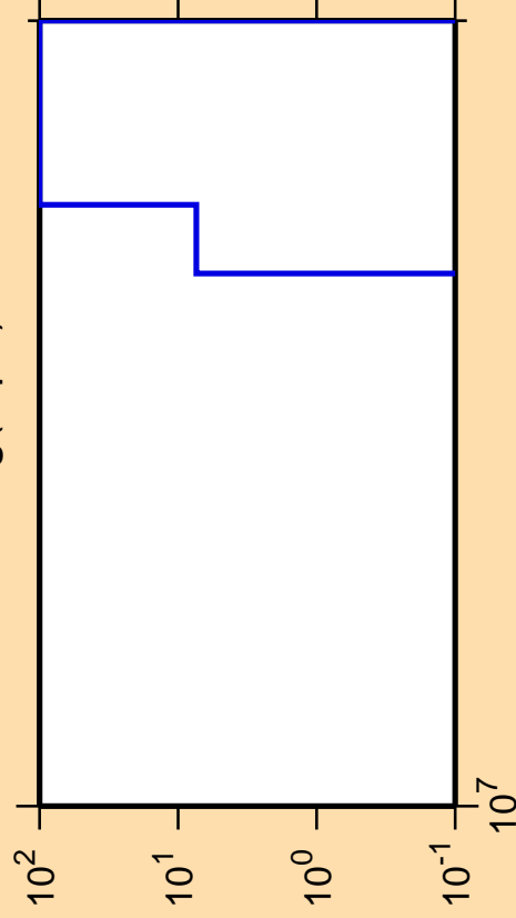
\Delta\sigma/\sigma vs. E for ^{207}\text{Hg}(n,p\alpha)
