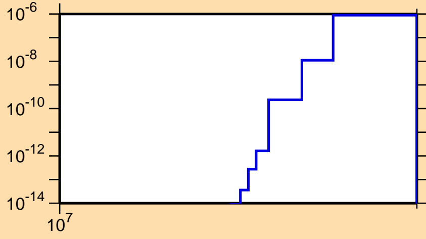
\sigma vs. E for ^{207}\text{Hg}(n,nt)
