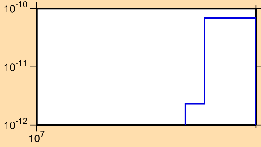
\sigma vs. E for ^{207}\text{Hg}(n,p\alpha)
