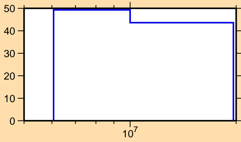
\Delta\sigma/\sigma vs. E for ^{207}\text{Hg}(n,p)
