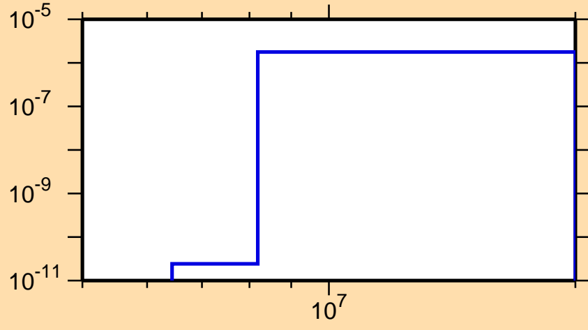
\sigma vs. E for ^{207}\text{Hg}(n,n\alpha)
