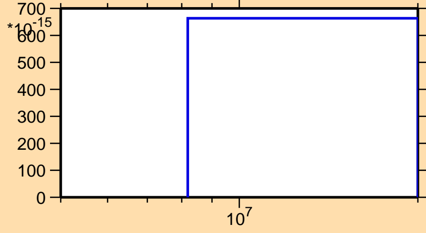
\sigma vs. E for ^{207}\text{Hg}(n,p\alpha)
