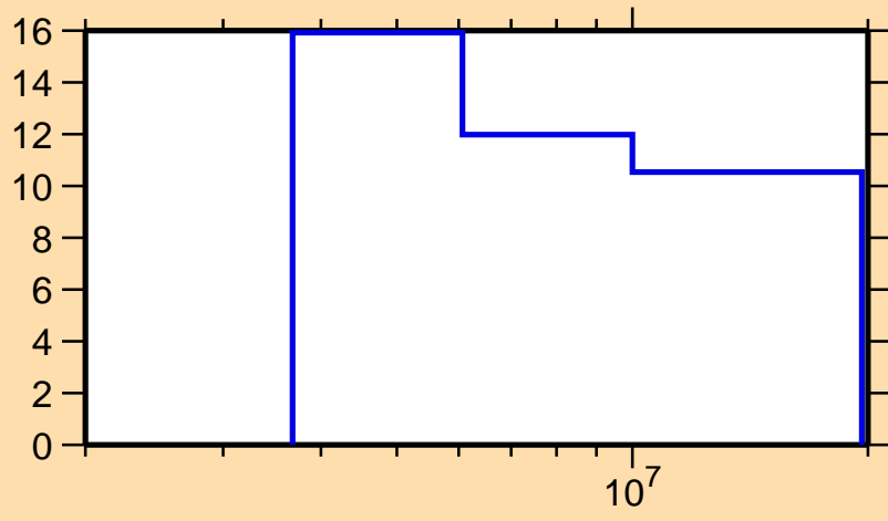
\Delta\sigma/\sigma vs. E for ^{208}\text{Hg}(n,\text{nonel.})
