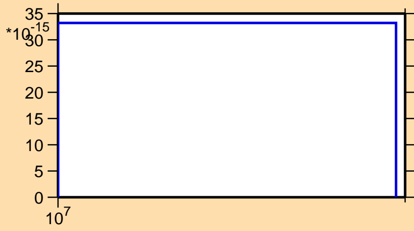
\sigma vs. E for ^{208}\text{Hg}(n,3n\alpha)
