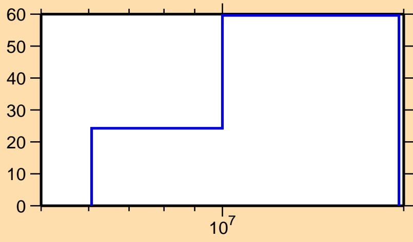
\Delta\sigma/\sigma vs. E for ^{208}\text{Hg}(n,2n)
