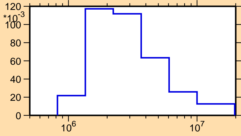
\sigma vs. E for ^{208}\text{Hg}(n,n_2)
