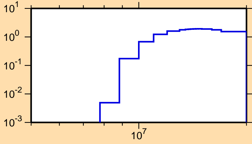
\sigma vs. E for ^{209}\text{Hg}(n,3n)
