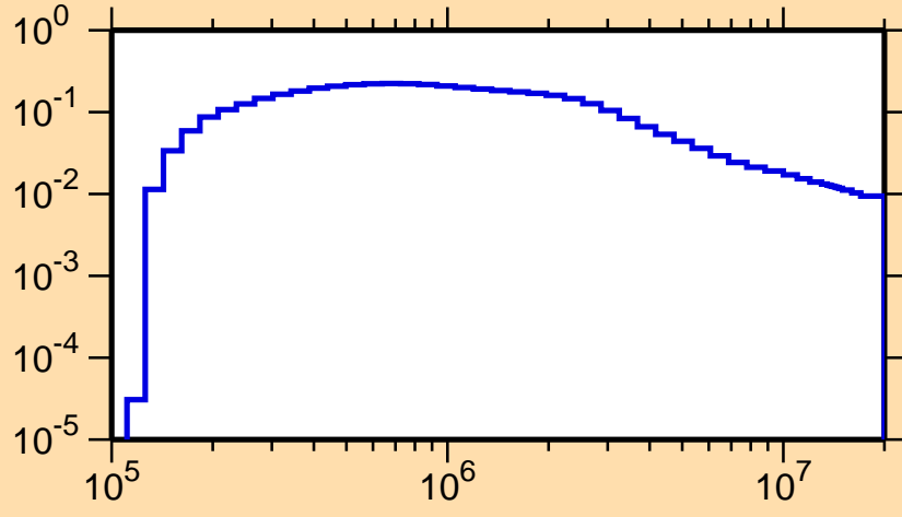
\sigma vs. E for ^{209}\text{Hg}(n,n_1)
