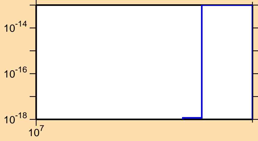
\sigma vs. E for ^{209}\text{Hg} (mt 11)
