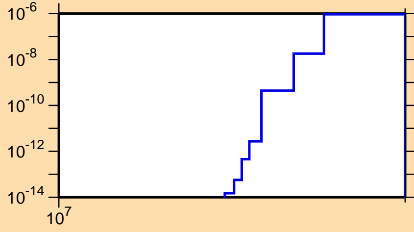
\sigma vs. E for ^{209}\text{Hg}(n,\text{nd})
