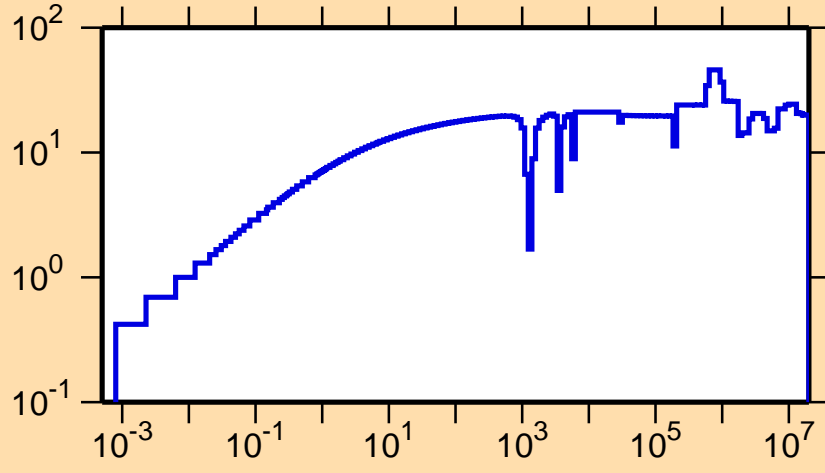
\Delta\sigma/\sigma vs. E for ^{209}\text{Hg}(n,\text{tot.})
