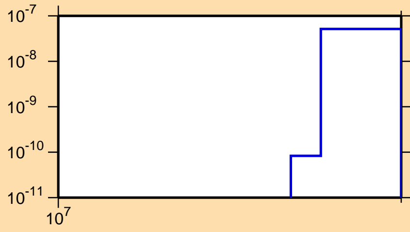
\sigma vs. E for ^{209}\text{Hg}(n,2np)
