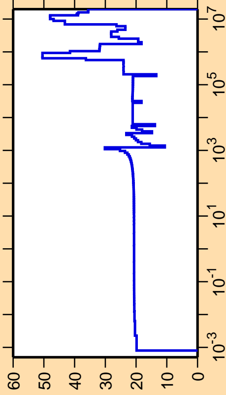
\Delta\sigma/\sigma vs. E for ^{209}\text{Hg}(n,\text{el.})
