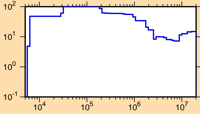
\Delta\sigma/\sigma vs. E for ^{209}\text{Hg}(n,\text{nonel.})
