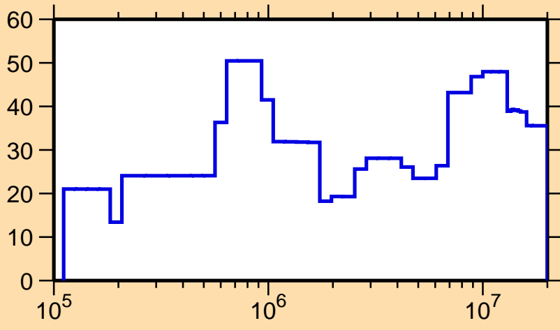
\Delta\sigma/\sigma vs. E for ^{209}\text{Hg}(n,\text{el.})
