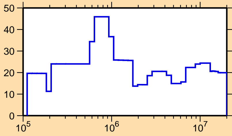
\Delta\sigma/\sigma vs. E for ^{209}\text{Hg}(n,\text{tot.})
