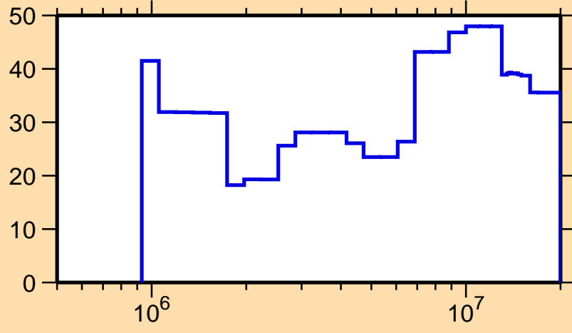
\Delta\sigma/\sigma vs. E for ^{209}\text{Hg}(n,\text{el.})
