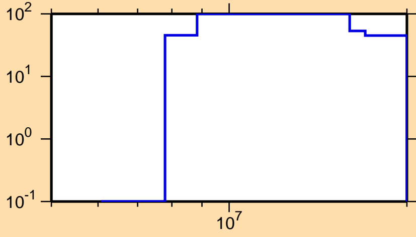
\Delta\sigma/\sigma vs. E for ^{209}\text{Hg}(n,p)
