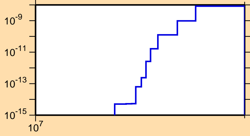
\sigma vs. E for ^{209}\text{Hg}(n,p\alpha)
