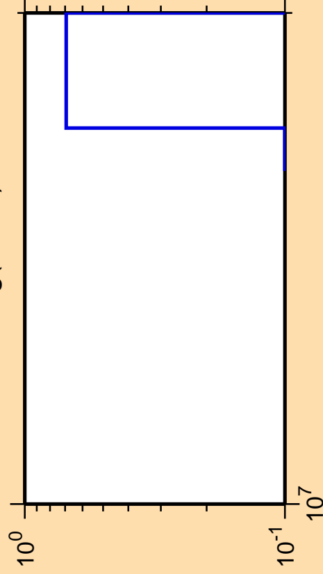
\Delta\sigma/\sigma vs. E for ^{209}\text{Hg} (mt 11)
