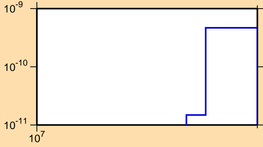
\sigma vs. E for ^{209}\text{Hg}(n,3n\alpha)
