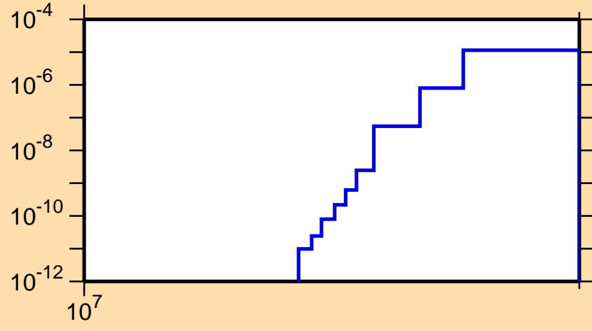
\sigma vs. E for ^{209}\text{Hg}(n,nt)
