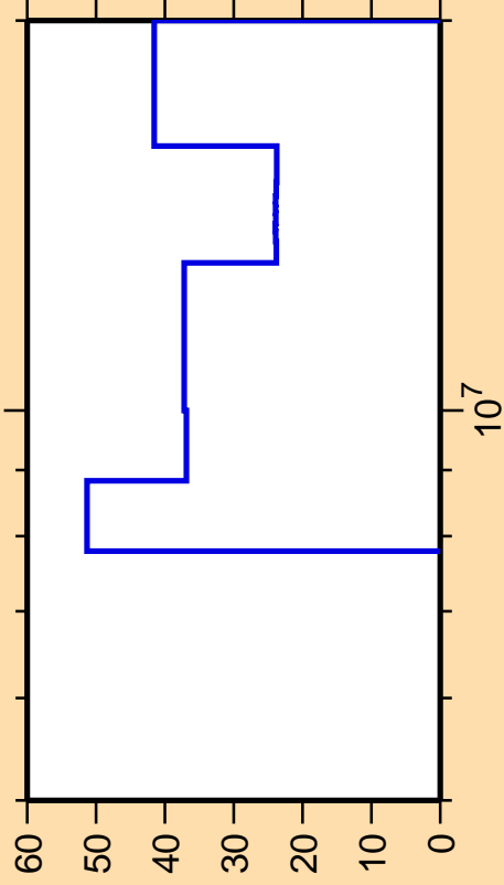
\Delta\sigma/\sigma vs. E for ^{209}\text{Hg}(n,3n)
