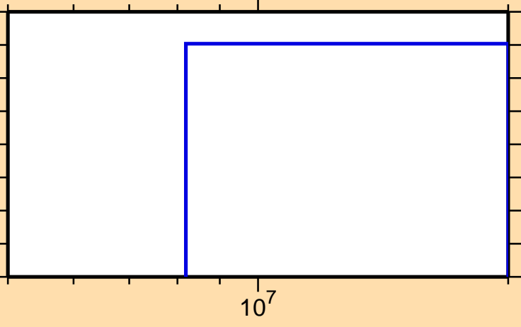
\sigma vs. E for ^{209}\text{Hg}(n,t)
