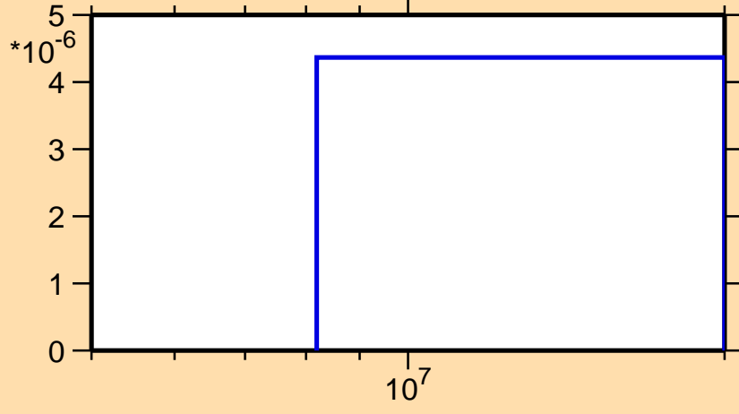
\sigma vs. E for ^{209}\text{Hg}(n,d)
