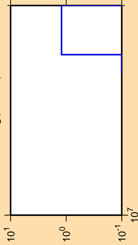
\Delta\sigma/\sigma vs. E for ^{210}\text{Hg}(\text{mt117})
