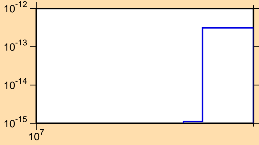
\sigma vs. E for ^{210}\text{Hg}(\text{mt117})
