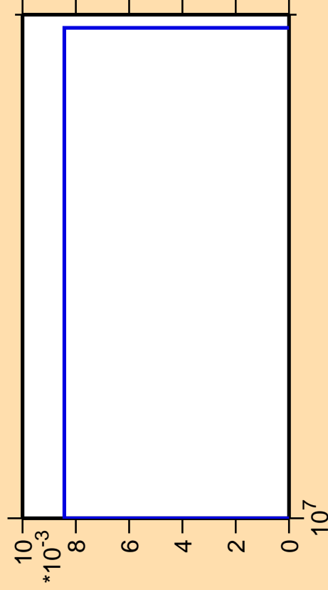
\Delta\sigma/\sigma vs. E for ^{210}\text{Hg} (mt117)
