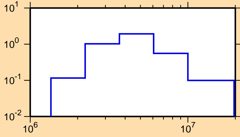
\sigma vs. E for ^{210}\text{Hg}(n,n\text{cont.})
