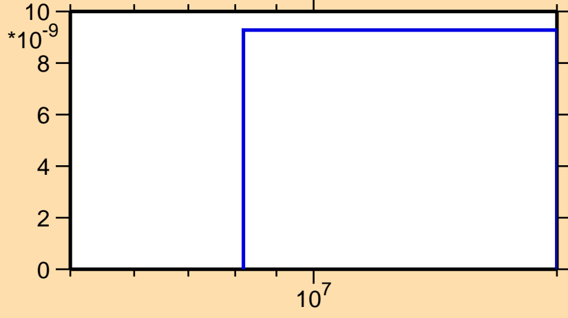
\sigma vs. E for ^{210}\text{Hg}(n,2n\alpha)
