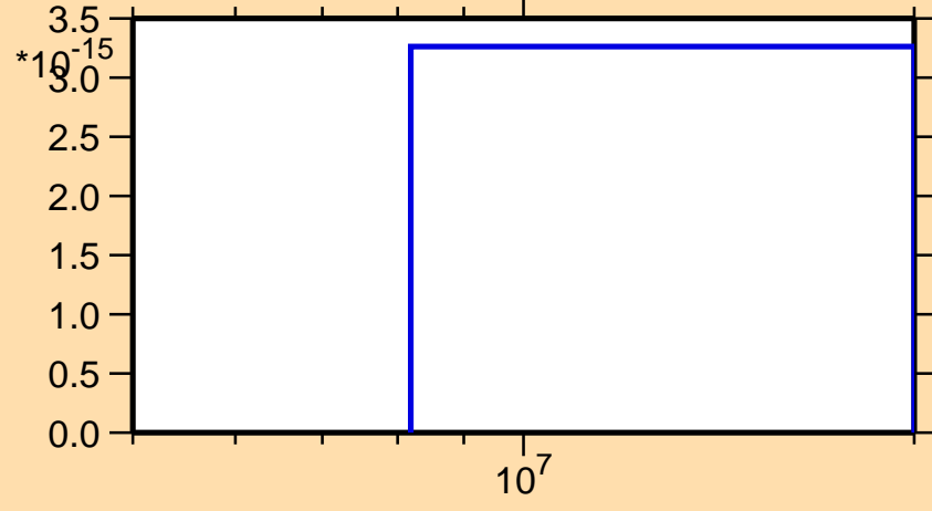
\sigma vs. E for ^{210}\text{Hg}(\text{mt117})
