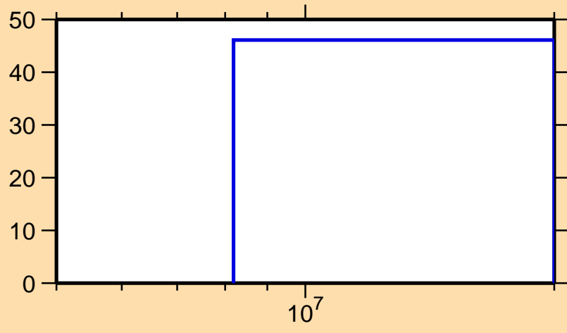
\Delta\sigma/\sigma vs. E for ^{210}\text{Hg}(n,p)
