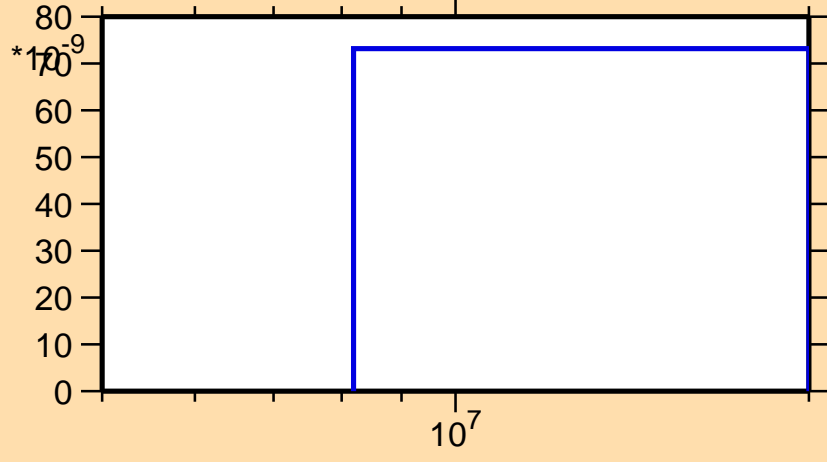
\sigma vs. E for ^{210}\text{Hg}(n,nt)
