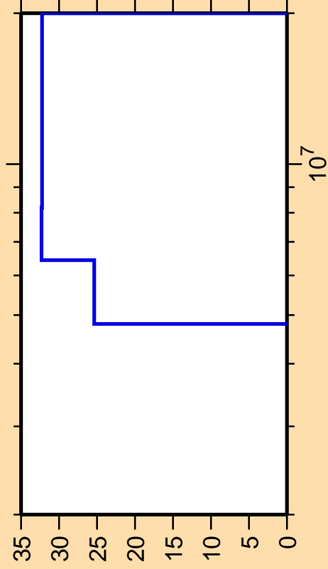
\Delta\sigma/\sigma vs. E for ^{210}\text{Hg}(n,n_1)
