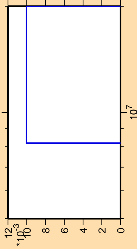
\Delta\sigma/\sigma vs. E for ^{210}\text{Hg}(\text{mt117})
