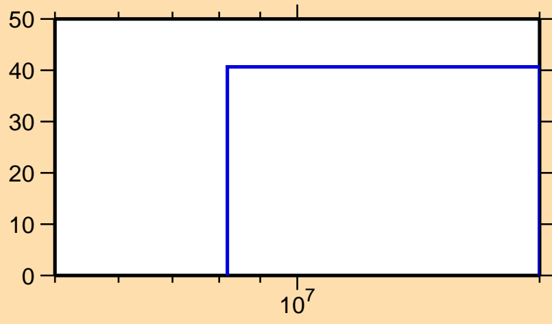
\Delta\sigma/\sigma vs. E for ^{210}\text{Hg}(n,ncont.)
