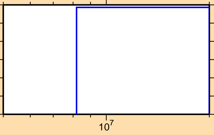
\sigma vs. E for ^{210}\text{Hg}(n,p)
