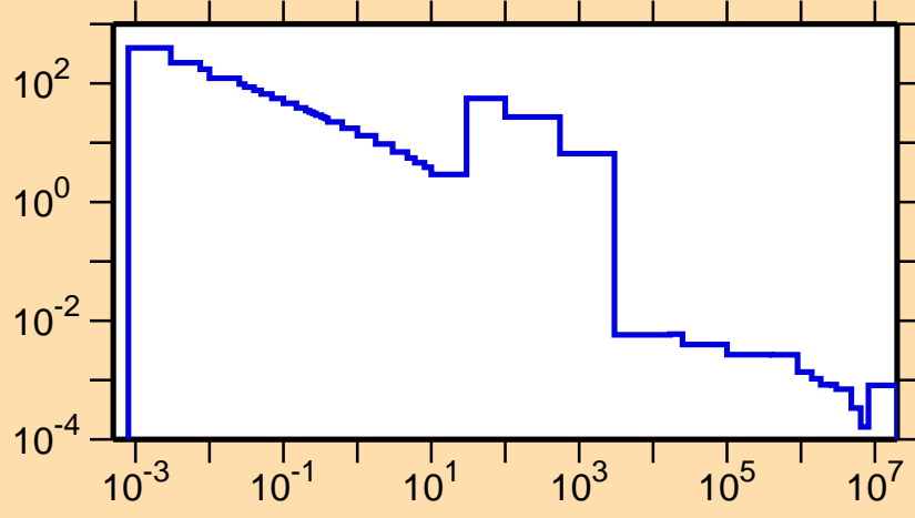
\sigma vs. E for ^{210}\text{Hg}(n,\gamma)
