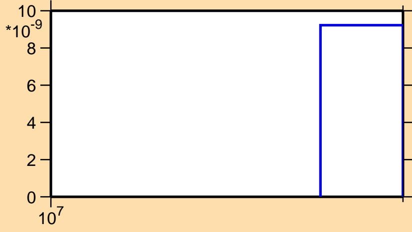
\sigma vs. E for ^{211}\text{Hg}(n,2np)
