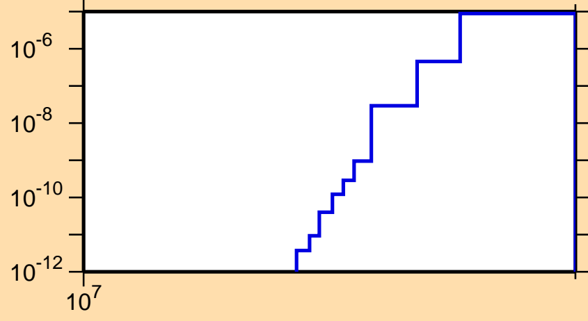
\sigma vs. E for ^{211}\text{Hg}(n,nt)
