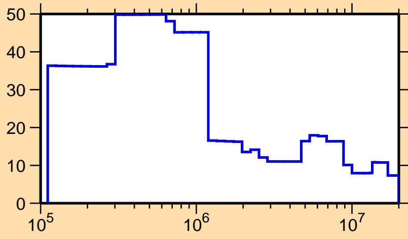
\Delta\sigma/\sigma vs. E for ^{211}\text{Hg}(n,\text{el.})
