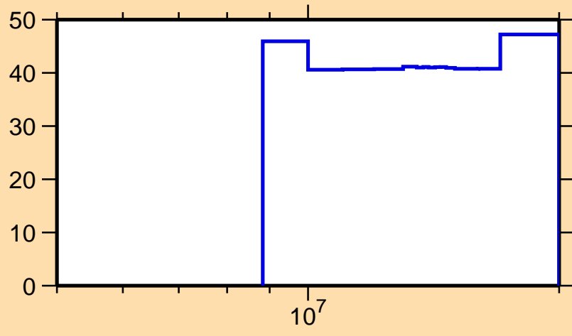
\Delta\sigma/\sigma vs. E for ^{211}\text{Hg}(n,n\text{cont.})
