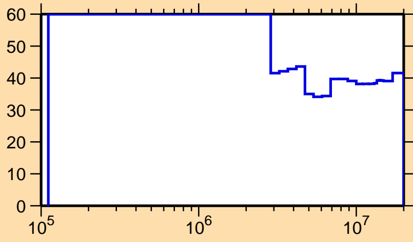
\Delta\sigma/\sigma vs. E for ^{211}\text{Hg}(n,n_1)
