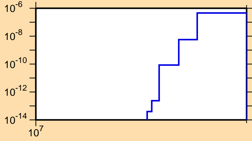
\sigma vs. E for ^{211}\text{Hg}(n,\text{nd})
