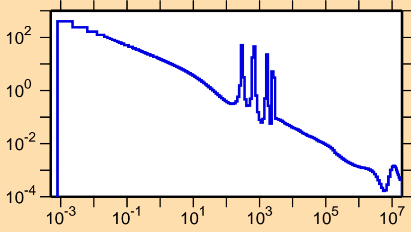
\sigma vs. E for ^{211}\text{Hg}(n,\gamma)
