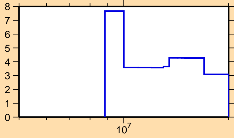
\Delta\sigma/\sigma vs. E for ^{211}\text{Hg}(n,\text{tot.})
