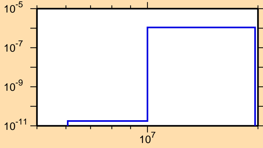
\sigma vs. E for ^{211}\text{Hg}(n,n\alpha)
