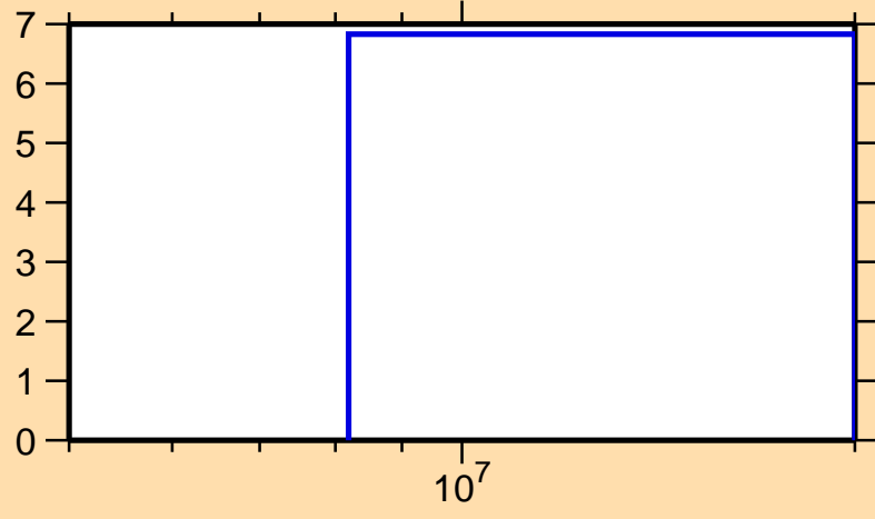
\Delta\sigma/\sigma vs. E for ^{211}\text{Hg}(n,\text{el.})
