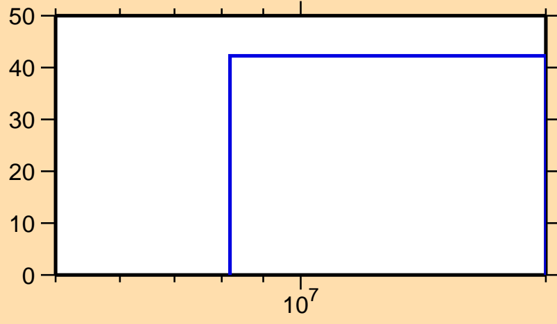
\Delta\sigma/\sigma vs. E for ^{211}\text{Hg}(n,ncont.)
