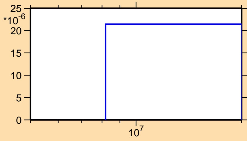
\sigma vs. E for ^{211}\text{Hg}(n,p)
