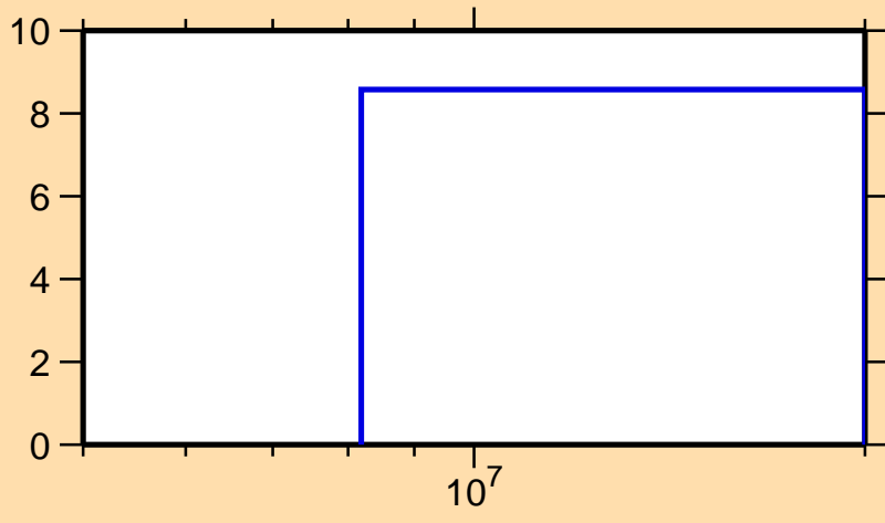
\Delta\sigma/\sigma vs. E for ^{211}\text{Hg}(n,\text{nonel.})
