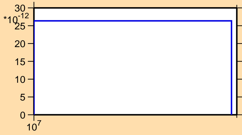
\sigma vs. E for ^{212}\text{Hg}(n,\text{nd})
