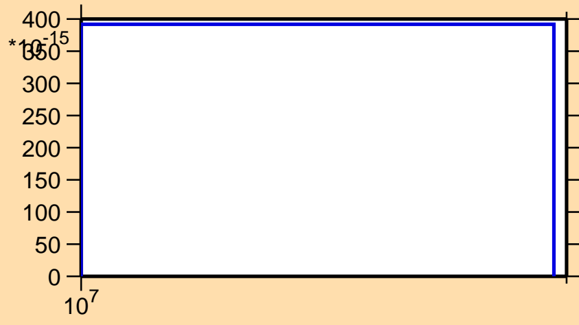
\sigma vs. E for ^{212}\text{Hg}(n,2np)
