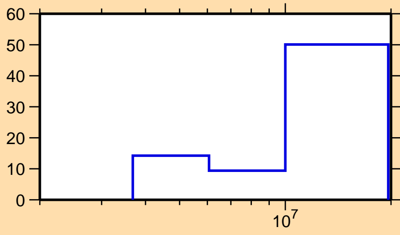
\Delta\sigma/\sigma vs. E for ^{212}\text{Hg}(n,2n)
