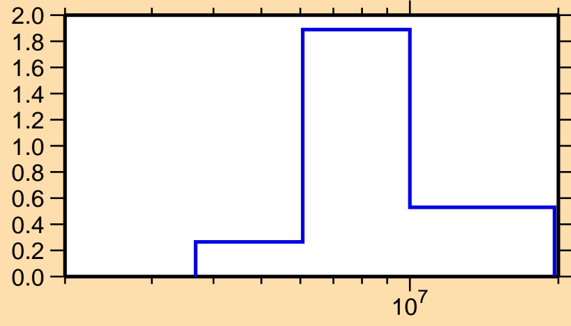
\sigma vs. E for ^{212}\text{Hg}(n,2n)
