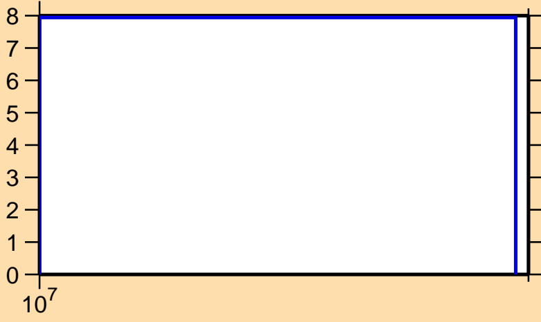
\Delta\sigma/\sigma vs. E for ^{212}\text{Hg}(n,el.)
