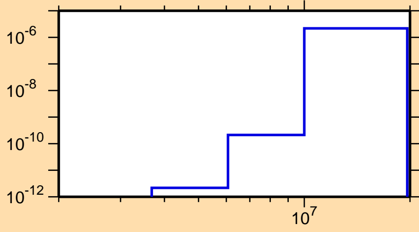
\sigma vs. E for ^{212}\text{Hg}(n,\alpha)
