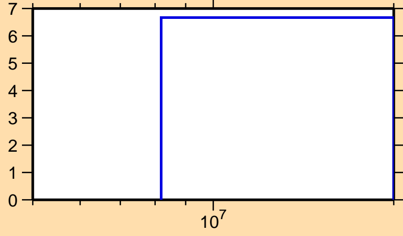
\Delta\sigma/\sigma vs. E for ^{212}\text{Hg}(n,\text{el.})
