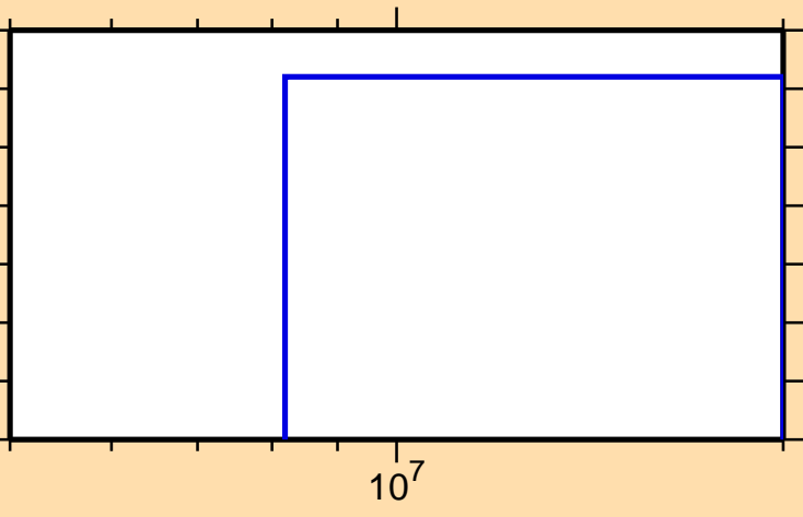
\sigma vs. E for ^{212}\text{Hg}(n,d)
