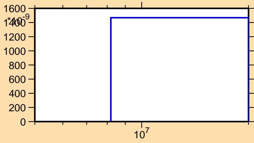
\sigma vs. E for ^{212}\text{Hg}(n,p)
