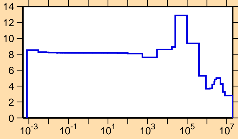
\sigma vs. E for ^{212}\text{Hg}(n,\text{el.})
