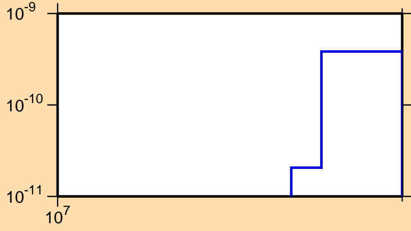
\sigma vs. E for ^{213}\text{Hg}(n,3n\alpha)
