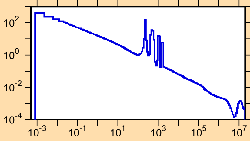
\sigma vs. E for ^{213}\text{Hg}(n,\gamma)
