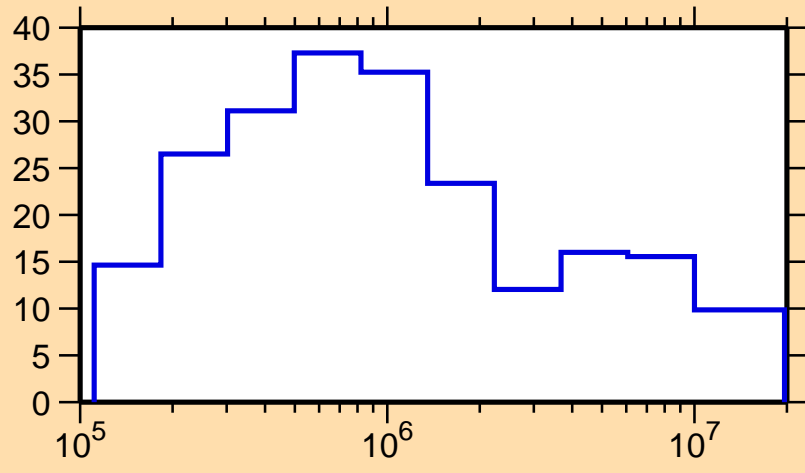
\Delta\sigma/\sigma vs. E for ^{213}\text{Hg}(n, el.)
