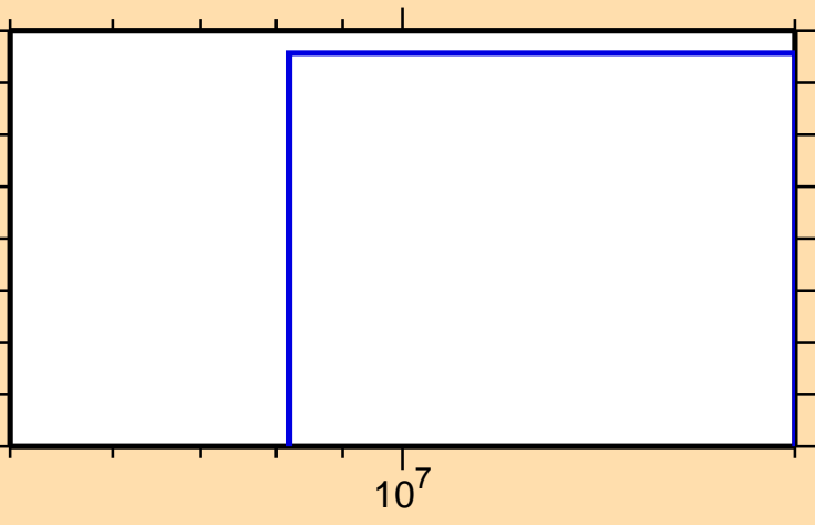
\sigma vs. E for ^{213}\text{Hg}(n,\text{nd})
