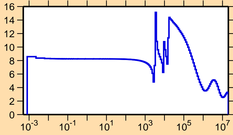
\sigma vs. E for ^{214}\text{Hg}(n,\text{el.})
