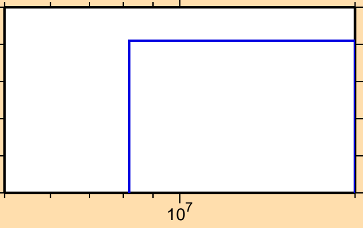
\sigma vs. E for ^{214}\text{Hg}(n,nt)
