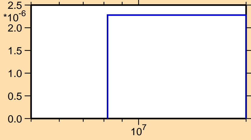
\sigma vs. E for ^{214}\text{Hg}(n,t)
