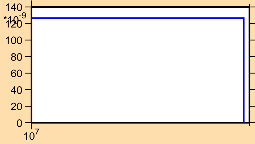
\sigma vs. E for ^{215}\text{Hg}(n,d)
