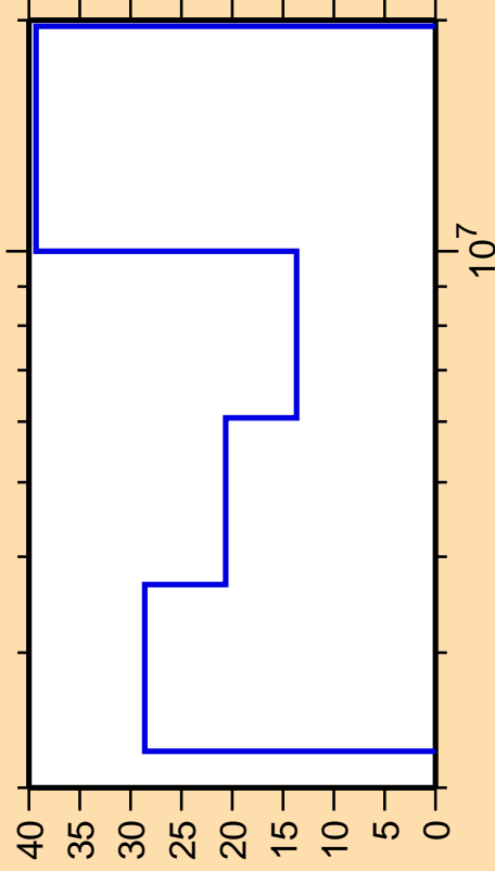
\Delta\sigma/\sigma vs. E for ^{215}\text{Hg}(n,2n)
