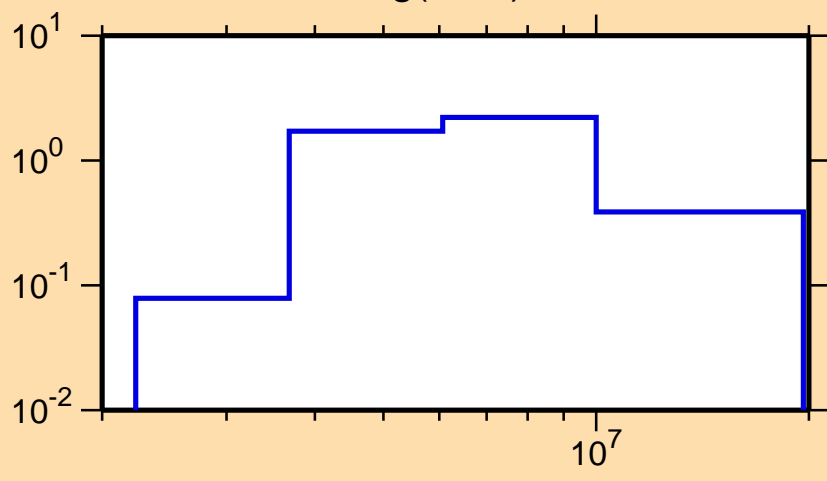
\sigma vs. E for ^{215}\text{Hg}(n,2n)
