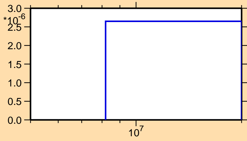
\sigma vs. E for ^{215}\text{Hg}(n,t)
