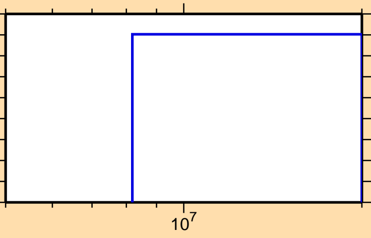
\sigma vs. E for ^{215}\text{Hg}(n,np)
