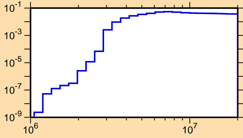
\sigma vs. E for ^{145}\text{Ho}(n,n\text{cont.})
