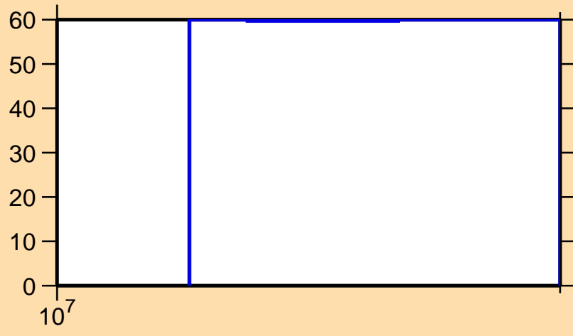
\Delta\sigma/\sigma vs. E for ^{145}\text{Ho}(n,2n)
