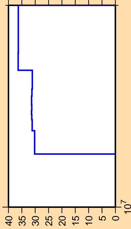
\Delta\sigma/\sigma vs. E for ^{145}\text{Ho}(n,n_1)
