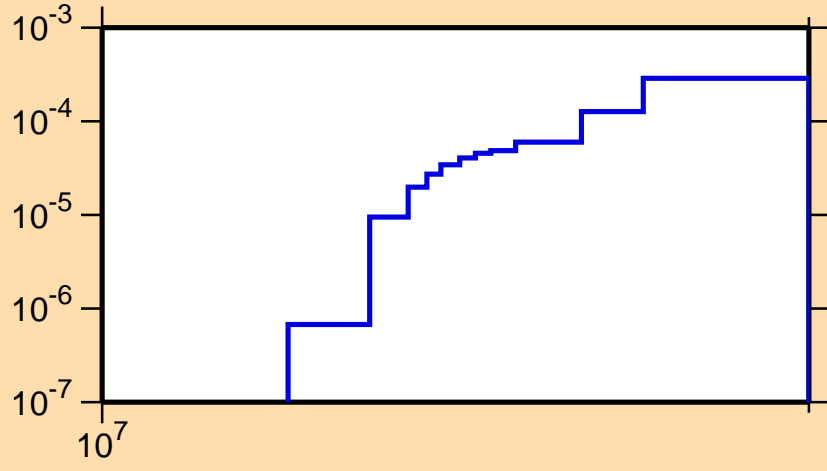
\sigma vs. E for ^{145}\text{Ho}(n,2n)
