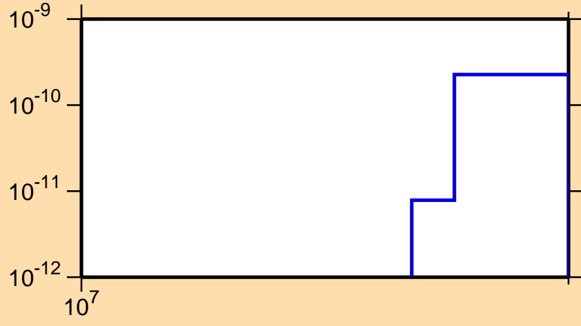
\sigma vs. E for ^{145}\text{Ho} (mt 34)
