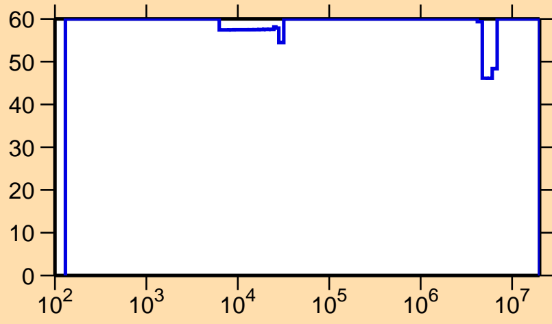
\Delta\sigma/\sigma vs. E for ^{145}\text{Ho}(n,\gamma)
