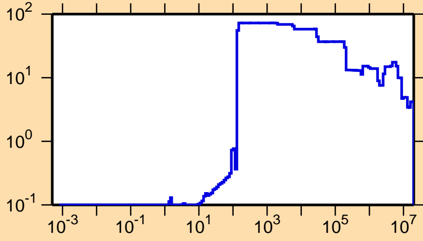
\Delta\sigma/\sigma vs. E for ^{145}\text{Ho}(n,\text{tot.})
