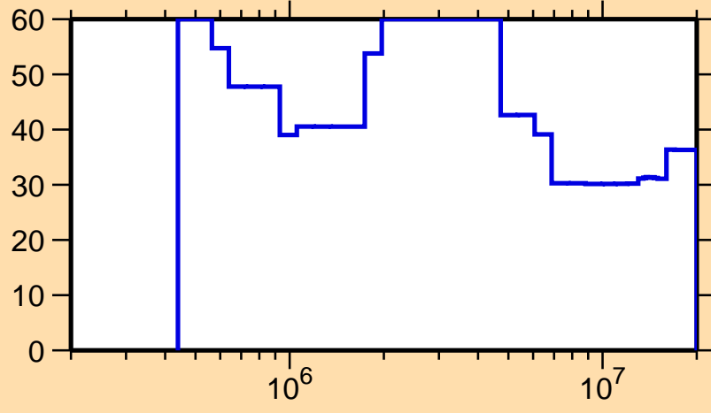
\Delta\sigma/\sigma vs. E for ^{145}\text{Ho}(n,n_1)
