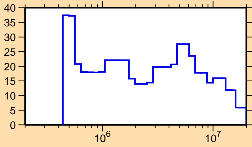
\Delta\sigma/\sigma vs. E for ^{145}\text{Ho}(n,\text{el.})
