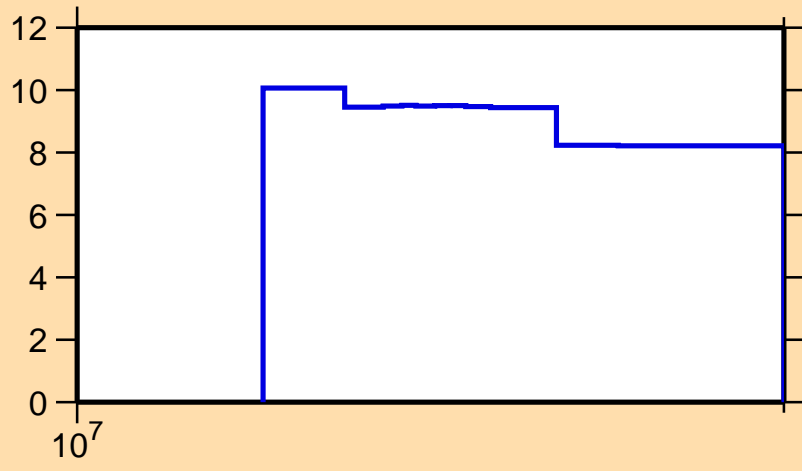
\Delta\sigma/\sigma vs. E for ^{145}\text{Ho}(n,\text{nonel.})
