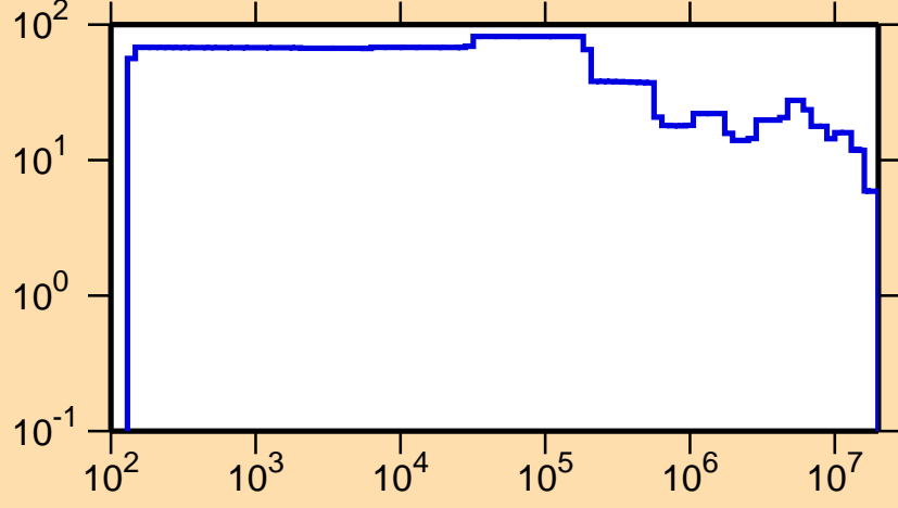
\Delta\sigma/\sigma vs. E for ^{145}\text{Ho}(n,\text{el.})
