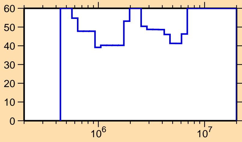
\Delta\sigma/\sigma vs. E for ^{145}\text{Ho}(n,\text{inel.})
