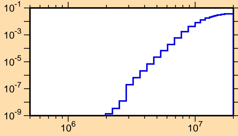
\sigma vs. E for ^{145}\text{Ho}(n,d)
