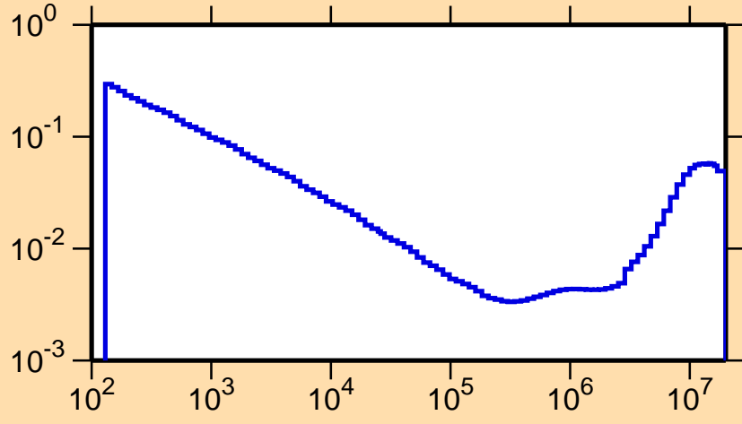
\sigma vs. E for ^{145}\text{Ho}(n,\alpha)
