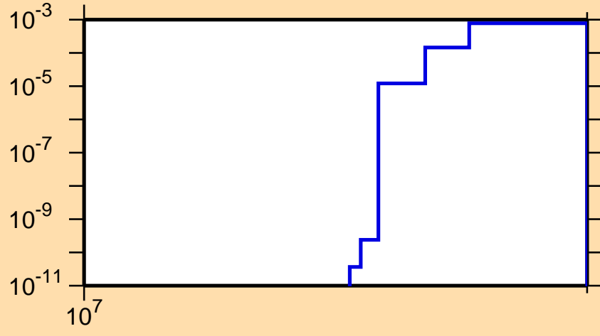
\sigma vs. E for ^{145}\text{Ho}(n,2np)
