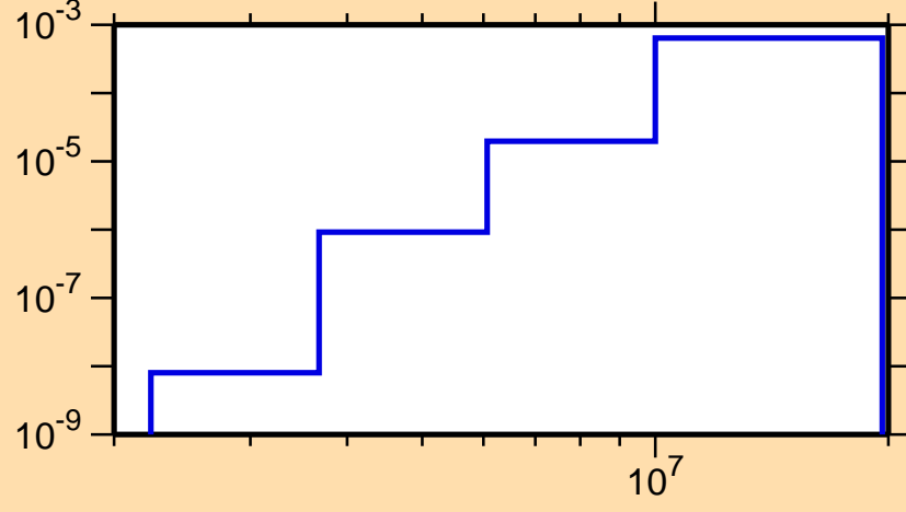
\sigma vs. E for ^{145}\text{Ho}(n,n\alpha)
