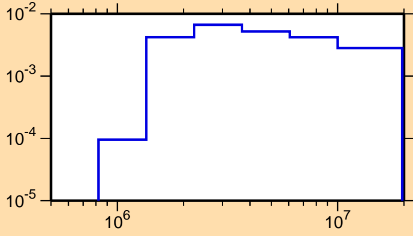
\sigma vs. E for ^{145}\text{Ho}(n,n_2)
