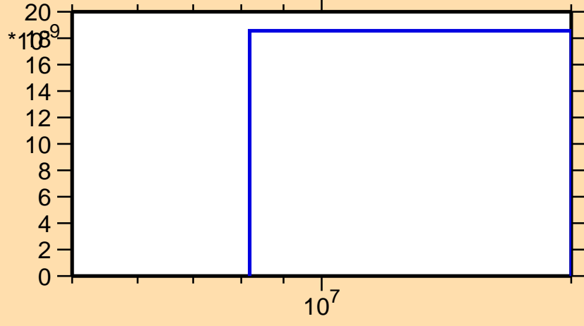
\sigma vs. E for ^{145}\text{Ho}(n,\text{nd})
