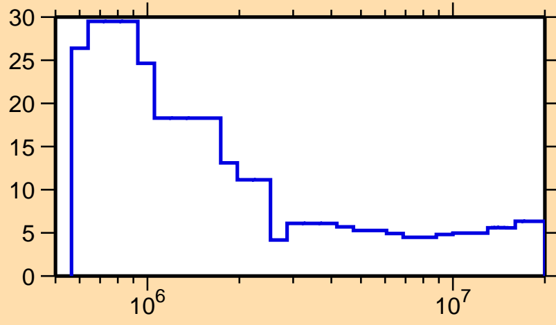
\Delta\sigma/\sigma vs. E for ^{147}\text{Ho}(n,\text{nonel.})
