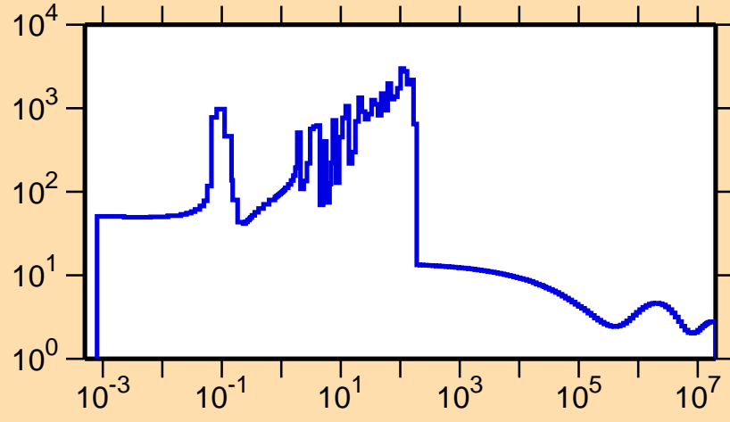
\sigma vs. E for ^{147}\text{Ho}(n,\text{el.})
