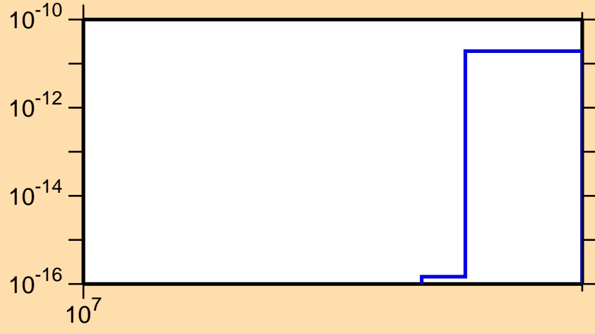
\sigma vs. E for ^{147}\text{Ho}(n,nt)
