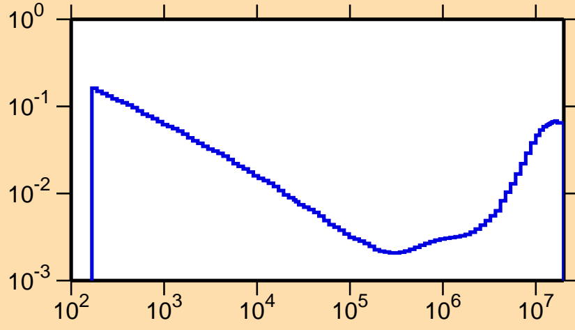
\sigma vs. E for ^{147}\text{Ho}(n,\alpha)
