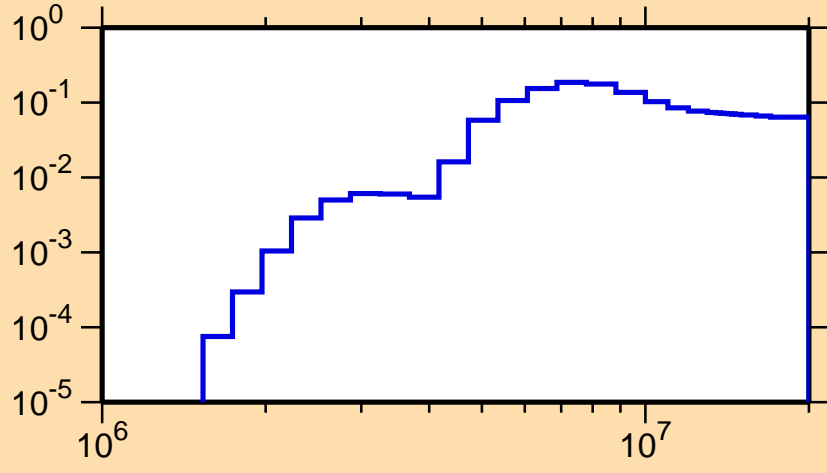
\sigma vs. E for ^{147}\text{Ho}(n,n\text{cont.})
