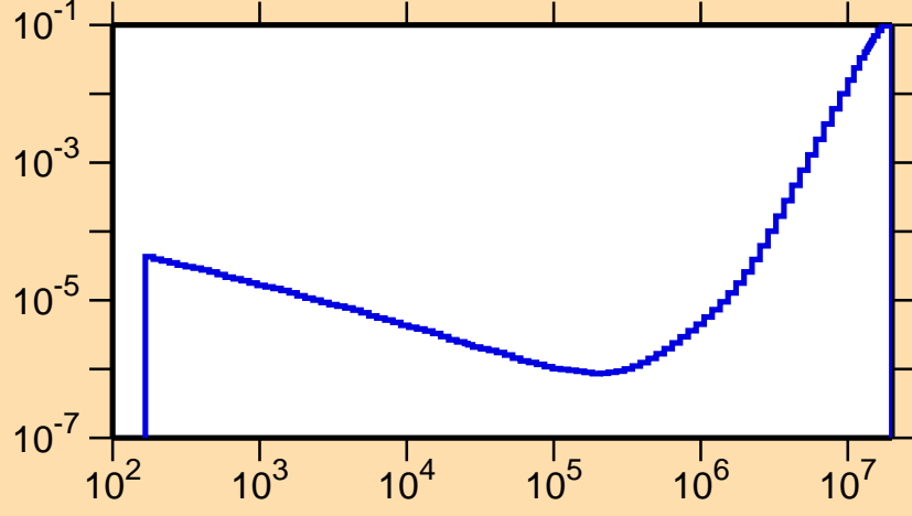
\sigma vs. E for ^{147}\text{Ho}(n,p\alpha)
