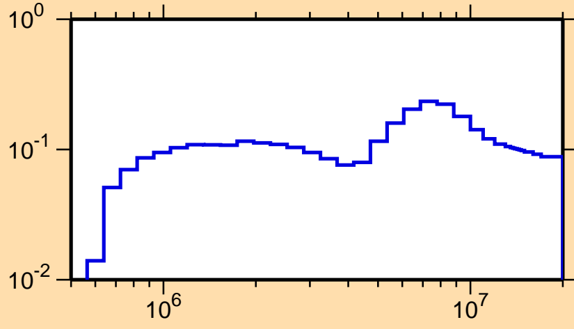
\sigma vs. E for ^{147}\text{Ho}(n,\text{inel.})
