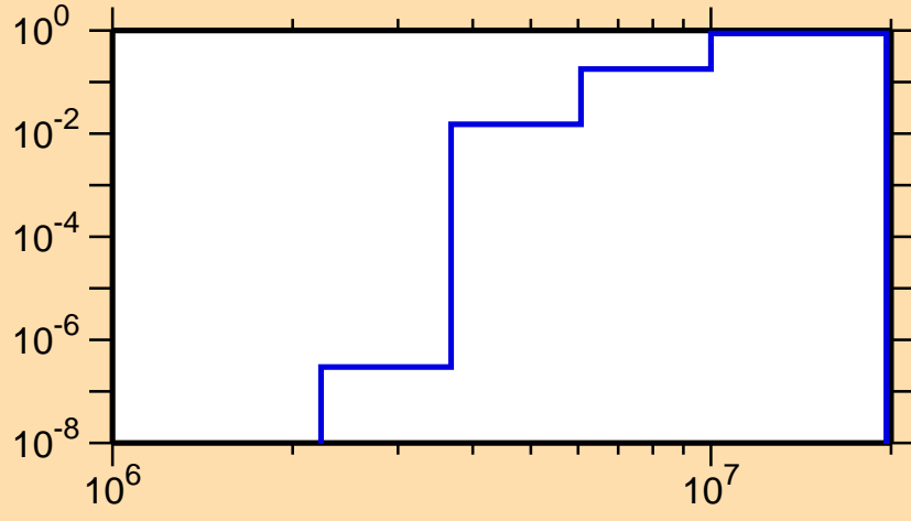
\sigma vs. E for ^{147}\text{Ho}(n,np)
