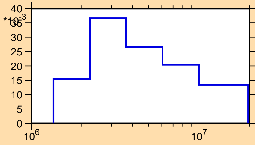
\sigma vs. E for ^{147}\text{Ho}(n,n_4)
