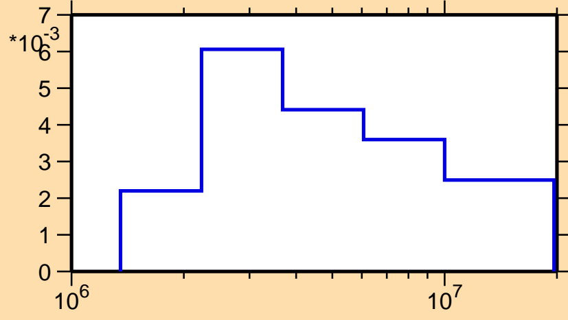
\sigma vs. E for ^{147}\text{Ho}(n,n_3)
