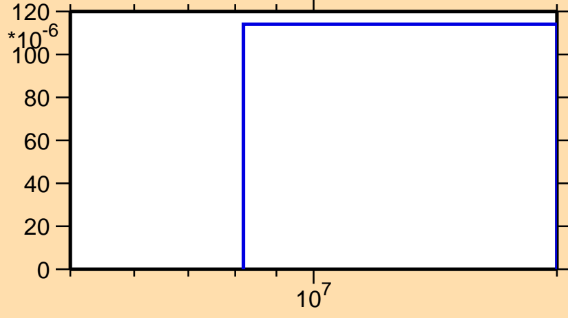
\sigma vs. E for ^{147}\text{Ho}(n,t)
