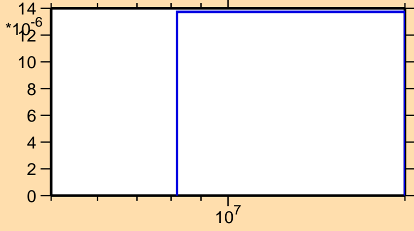
\sigma vs. E for ^{147}\text{Ho}(n,2np)
