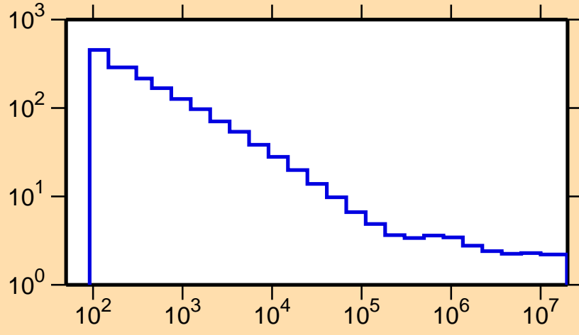
\sigma vs. E for ^{148}\text{Ho}(n,\text{nonel.})
