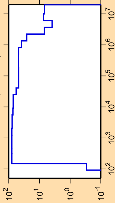
\Delta\sigma/\sigma vs. E for ^{148}\text{Ho}(n,\text{nonel.})
