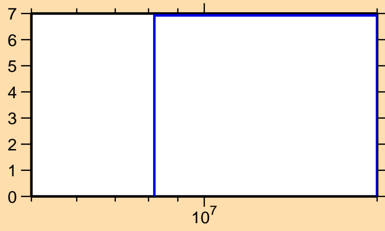
\Delta\sigma/\sigma vs. E for ^{148}\text{Ho}(n,\text{nonel.})
