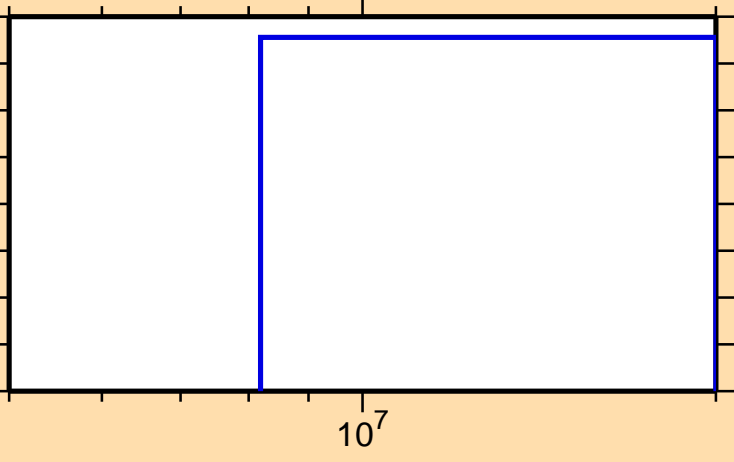
\sigma vs. E for ^{148}\text{Ho}(n,nt)
