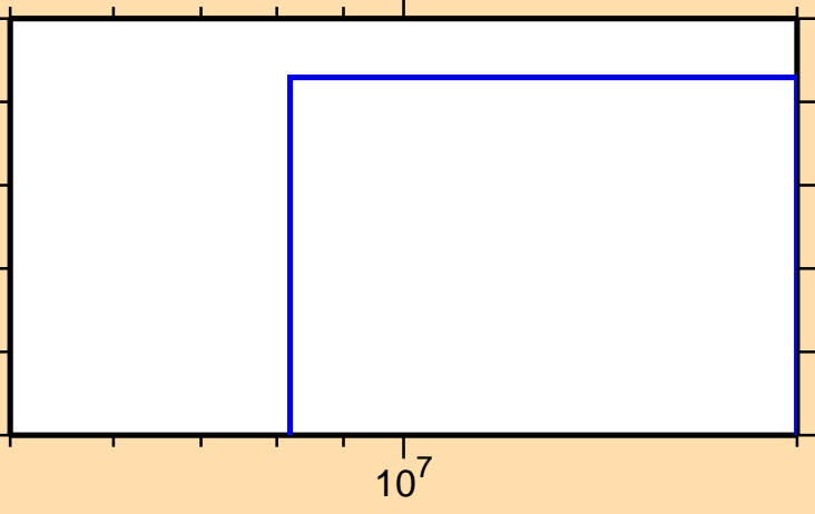
\sigma vs. E for ^{148}\text{Ho}(n,\text{nd})
