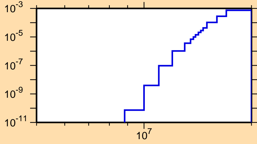
\sigma vs. E for ^{148}\text{Ho}(n,\text{pd})
