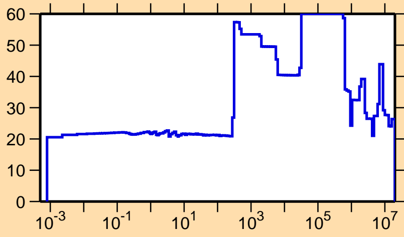
\Delta\sigma/\sigma vs. E for ^{148}\text{Ho}(n,\text{el.})
