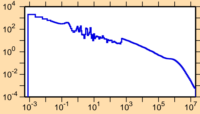
\sigma vs. E for ^{148}\text{Ho}(n,\gamma)
