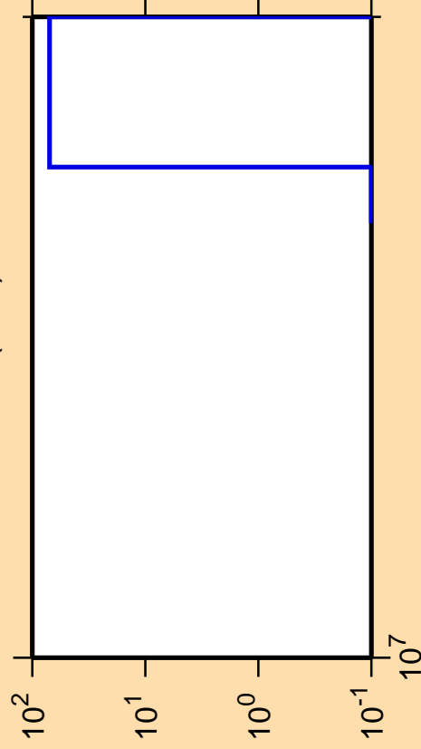
\Delta\sigma/\sigma vs. E for ^{148}\text{Ho}(n,nt)
