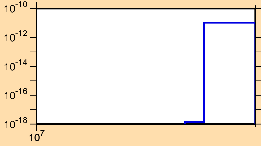
\sigma vs. E for ^{148}\text{Ho}(n,nt)
