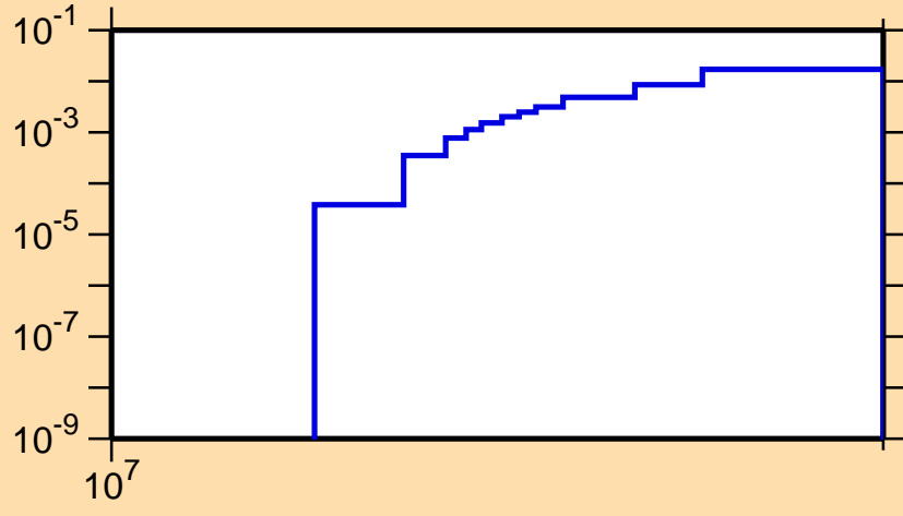
\sigma vs. E for ^{148}\text{Ho}(n,2np)
