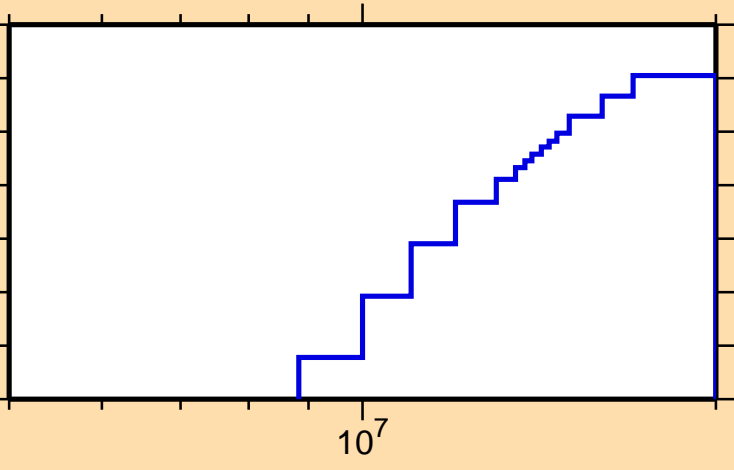
\sigma vs. E for ^{148}\text{Ho}(\text{mt117})
