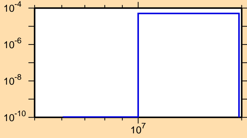
\sigma vs. E for ^{148}\text{Ho} (mt 45)
