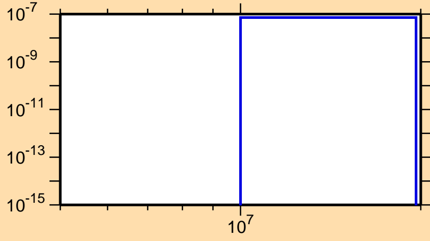
\sigma vs. E for ^{148}\text{Ho}(n,2n\alpha)
