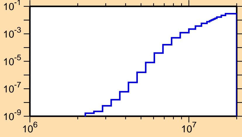
\sigma vs. E for ^{149}\text{Ho}(n,n\alpha)
