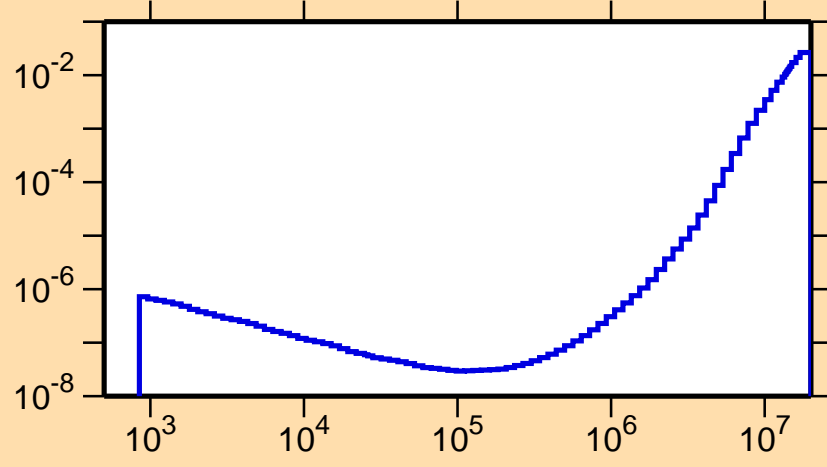
\sigma vs. E for ^{149}\text{Ho}(n, p\alpha)
