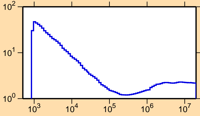
\sigma vs. E for ^{149}\text{Ho}(n,\text{nonel.})
