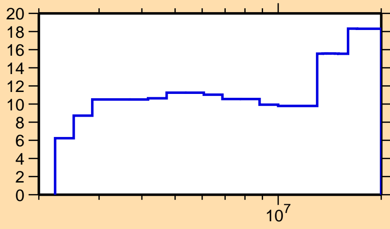
\Delta\sigma/\sigma vs. E for ^{149}\text{Ho}(n,n\text{onel.})
