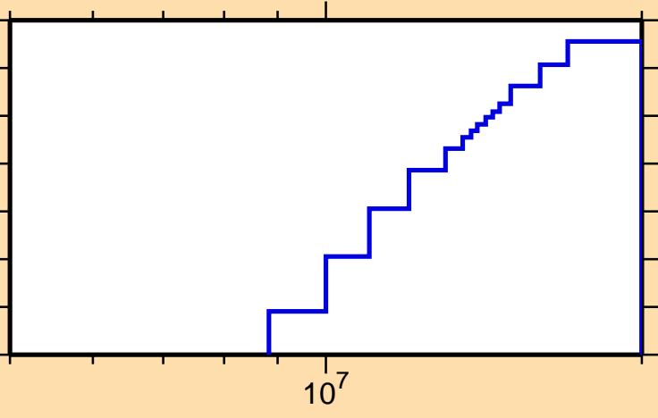
\sigma vs. E for ^{149}\text{Ho}(\text{mt117})
