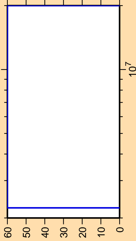
\Delta\sigma/\sigma vs. E for ^{149}\text{Ho}(n,n\text{cont.})
