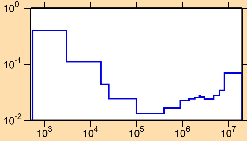
\sigma vs. E for ^{149}\text{Ho}(n,\alpha)
