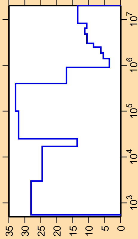
\Delta\sigma/\sigma vs. E for ^{149}\text{Ho}(n,\text{nonel.})
