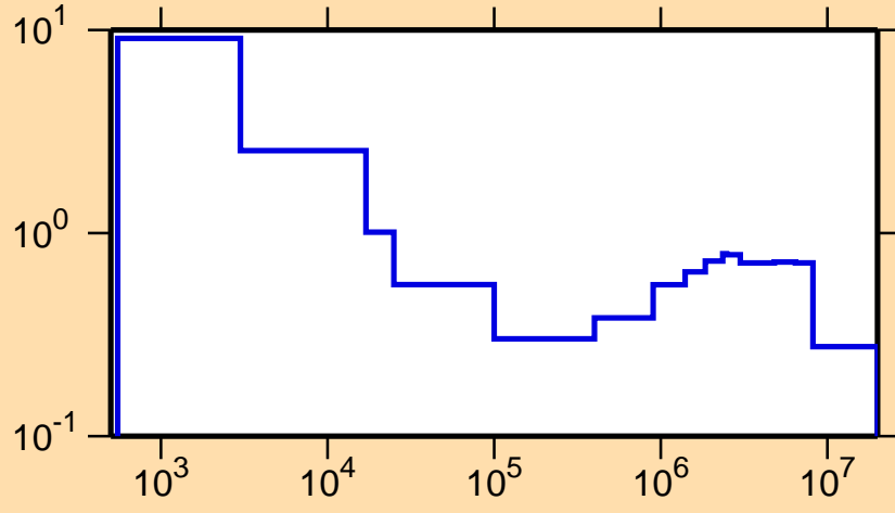
\sigma vs. E for ^{149}\text{Ho}(n,p)
