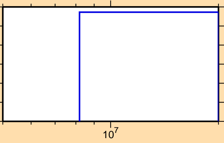
\sigma vs. E for ^{149}\text{Ho}(n,2n\alpha)
