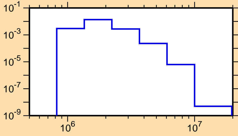
\sigma vs. E for ^{150}\text{Ho}(n,n_4)
