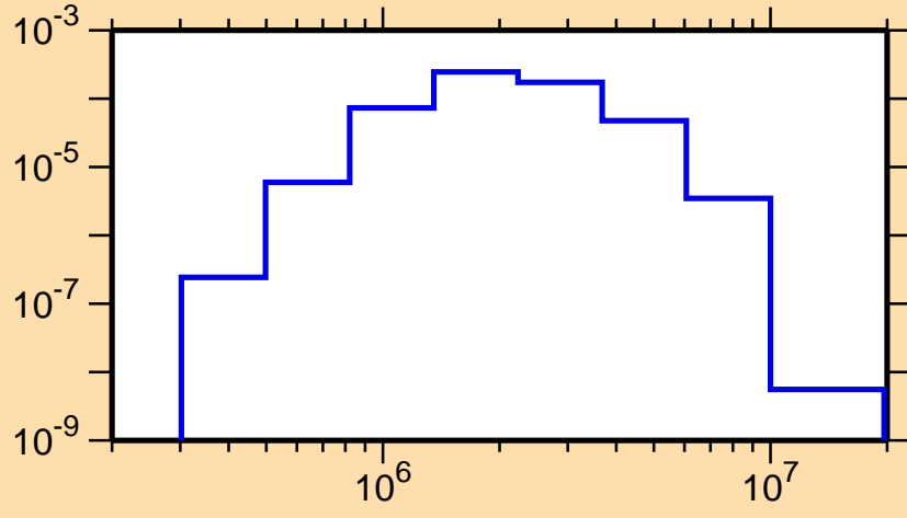
\sigma vs. E for ^{150}\text{Ho}(n,n_2)
