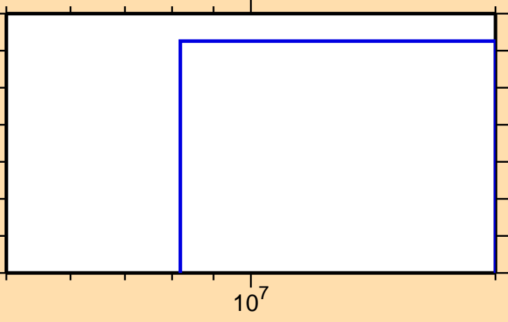
\sigma vs. E for ^{150}\text{Ho}(n,\text{nd})
